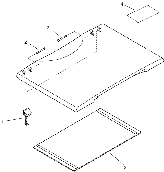
FIGURE 160 COPYBOARD COVER ASSEMBLY(ZTY,MTC,PVZ, QTL,UVB,UVC,UVD,UVE,ZTW,UMA,QRE)
