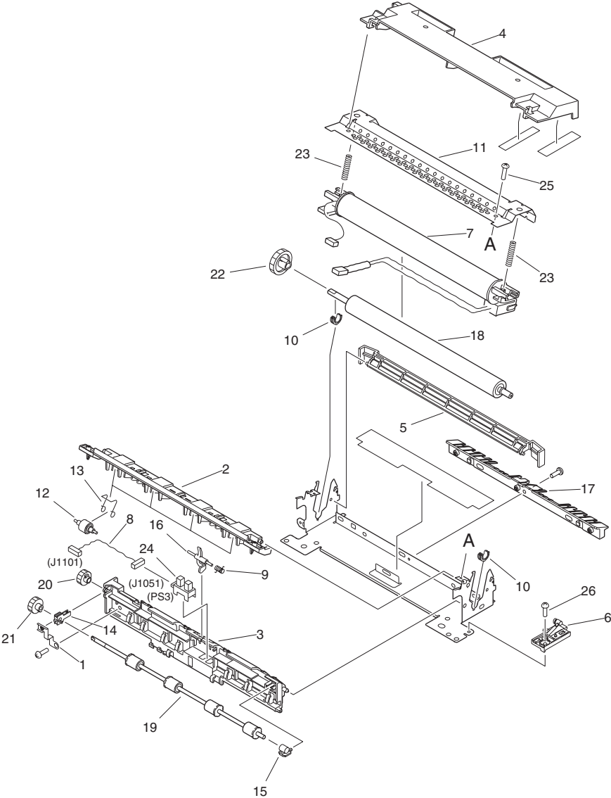
FIGURE 810 FIXING ASSEMBLY
