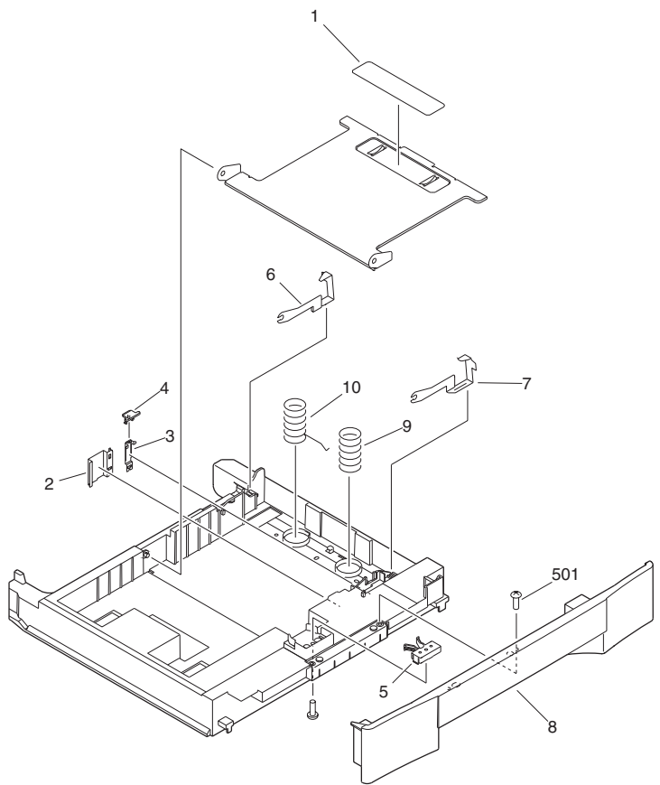
FIGURE 301 CASSETTE(QTL,UVB,UTC,UVD,UVE,UTM,UVF,UVG UVH,UVJ,UMA,UNA,UPA)
