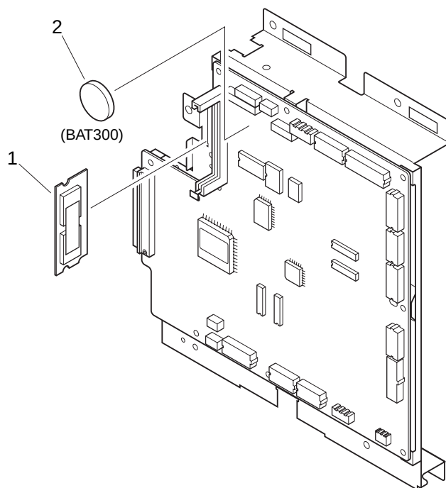
FIGURE 930 DC CONTROLLER PCB ASSEMBLY
