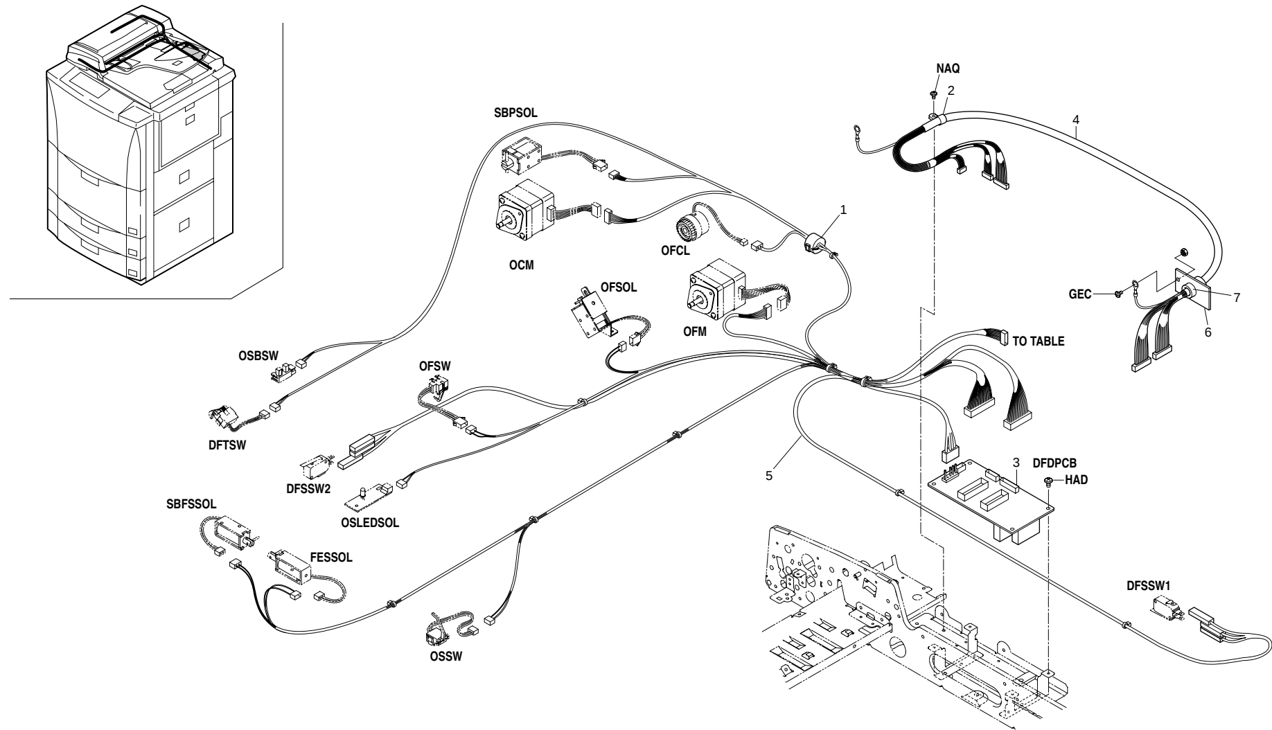
FIG.44 ELECTRICAL COMPONENTS (DF)
