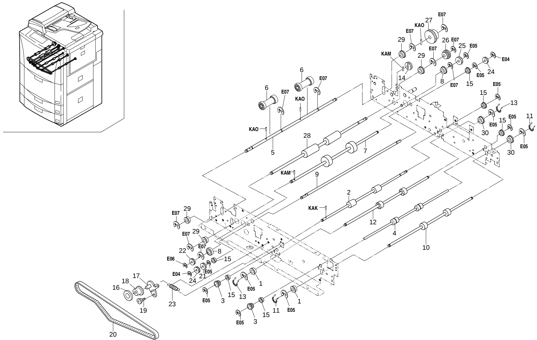
FIG.29 DUPLEX UNIT III
