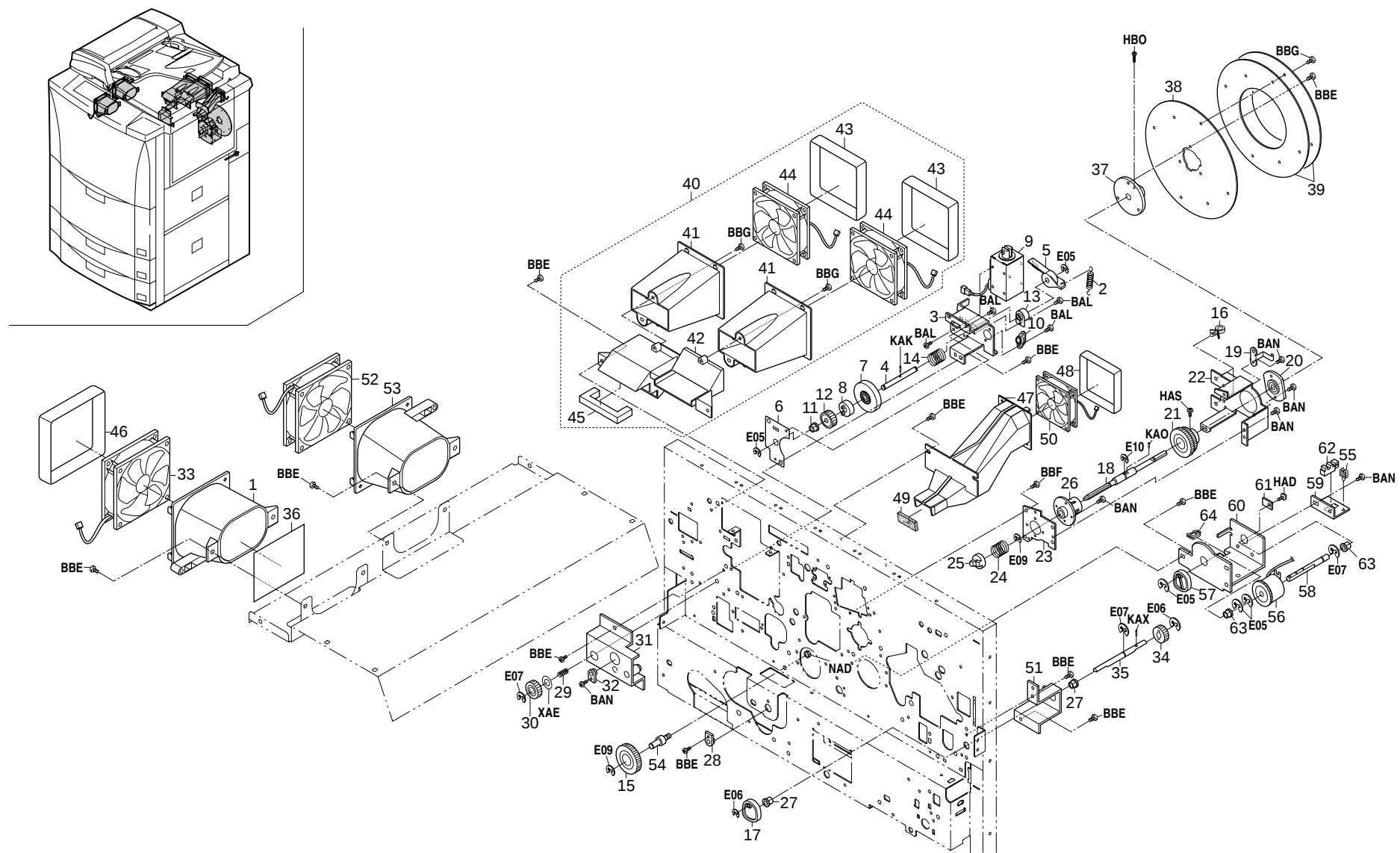
FIG.25 DRIVING, COOLING SECTION II
