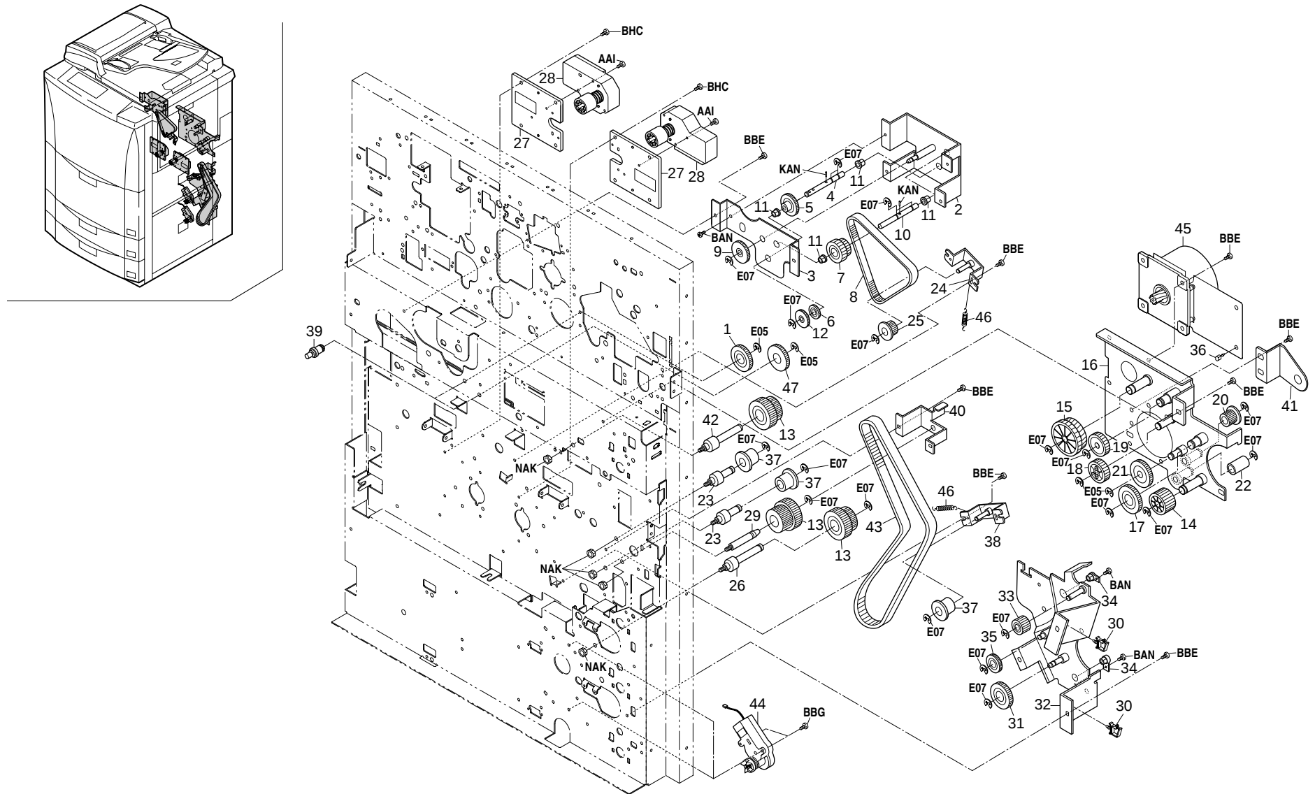
FIG.26 DRIVING, COOLING SECTION III
