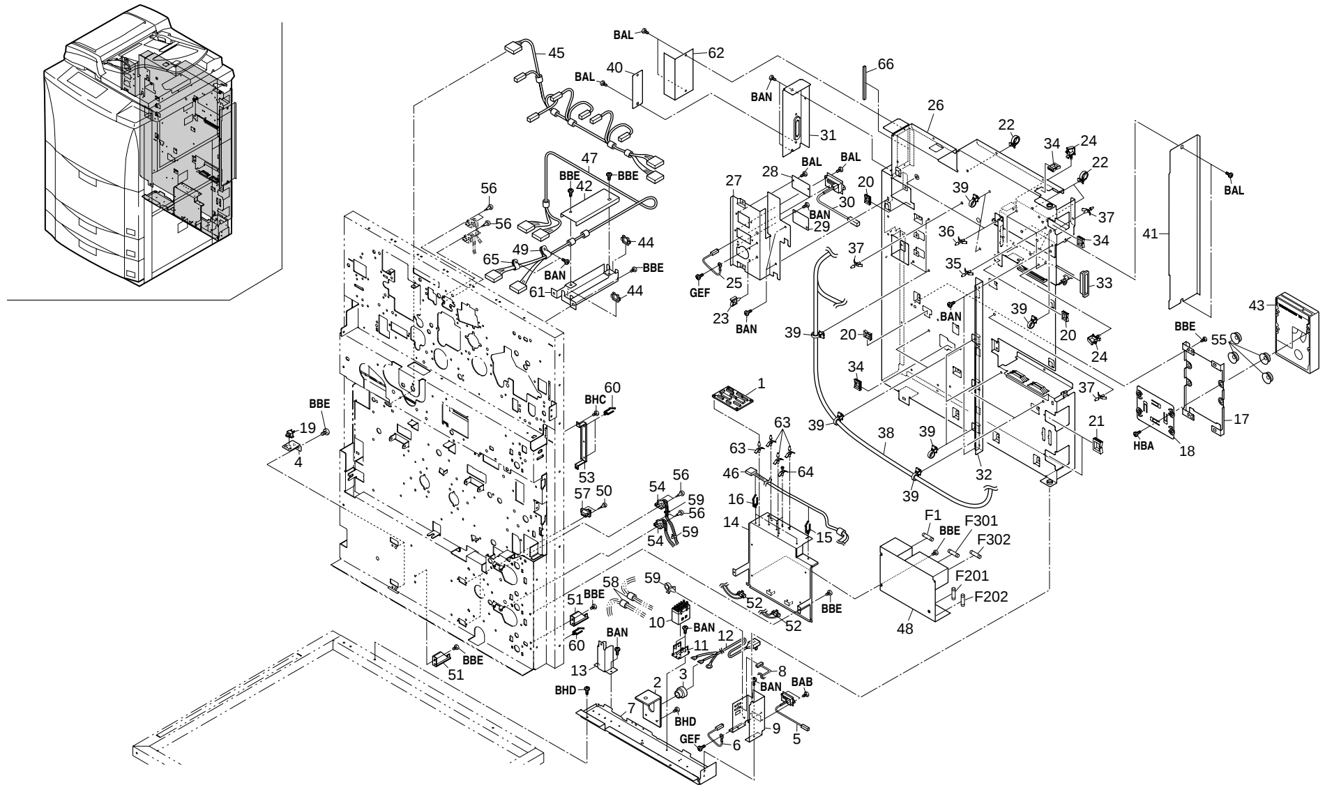
FIG.32 ELECTRICAL COMPONENTS I (120V)
