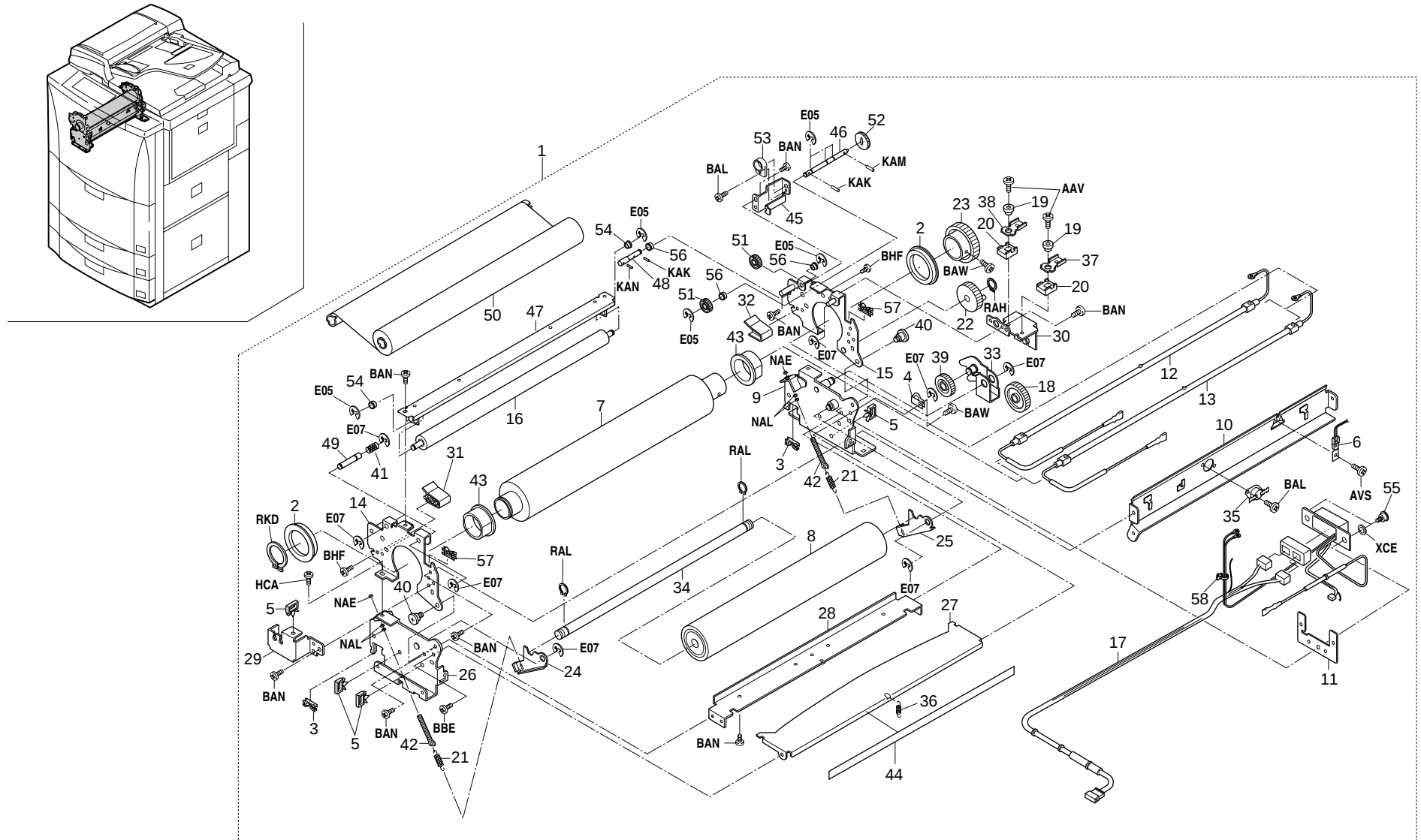
FIG.23 FIXING SECTION II
