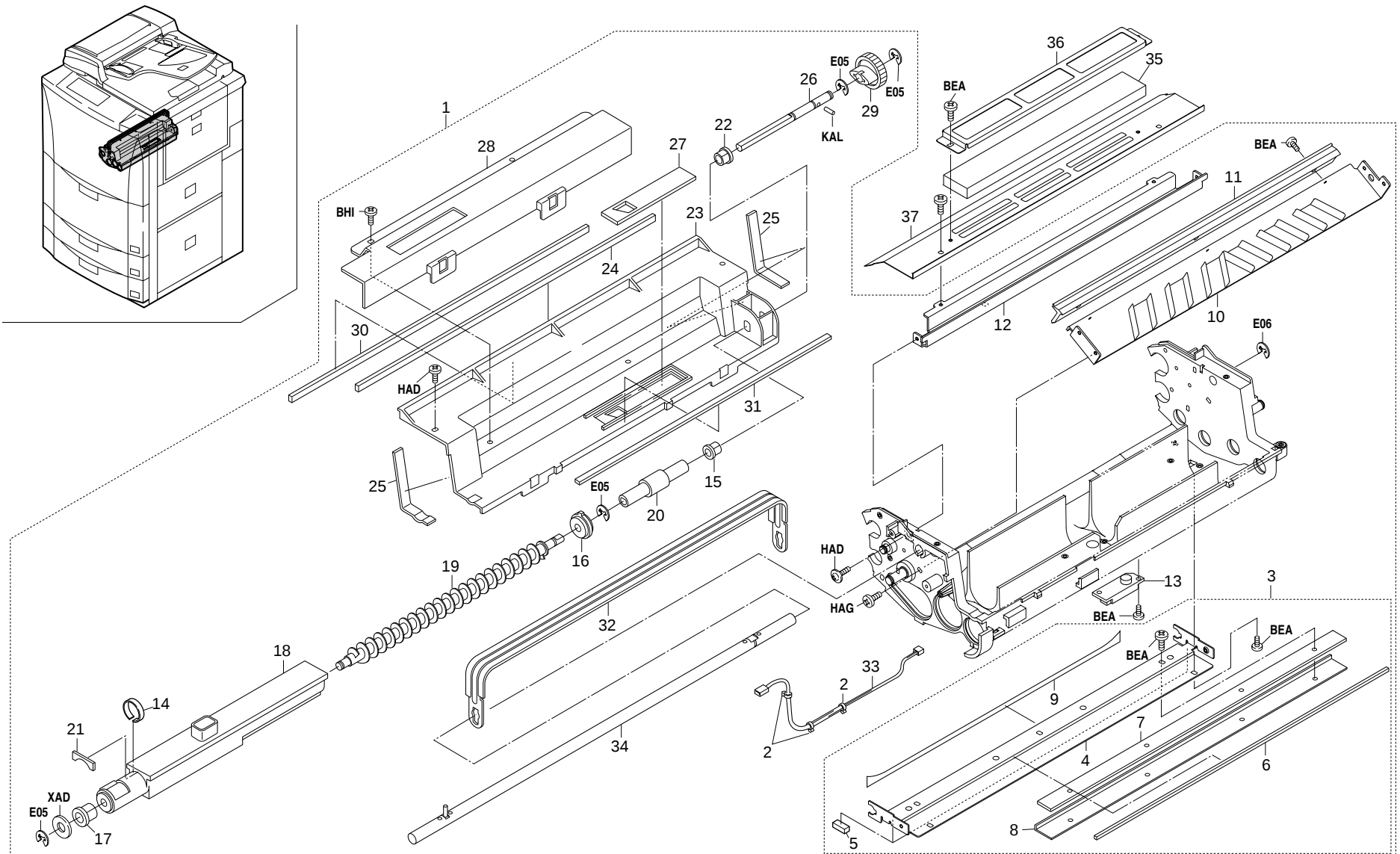
FIG.17 DEVELOPING SECTION I
