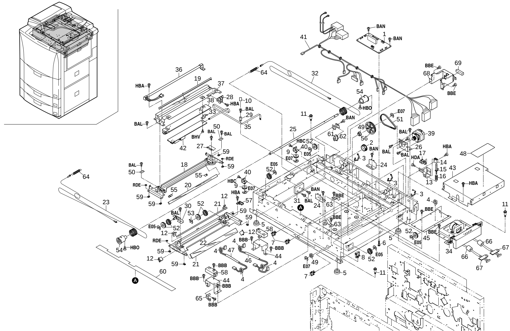
FIG.13 OPTICAL SECTION I
