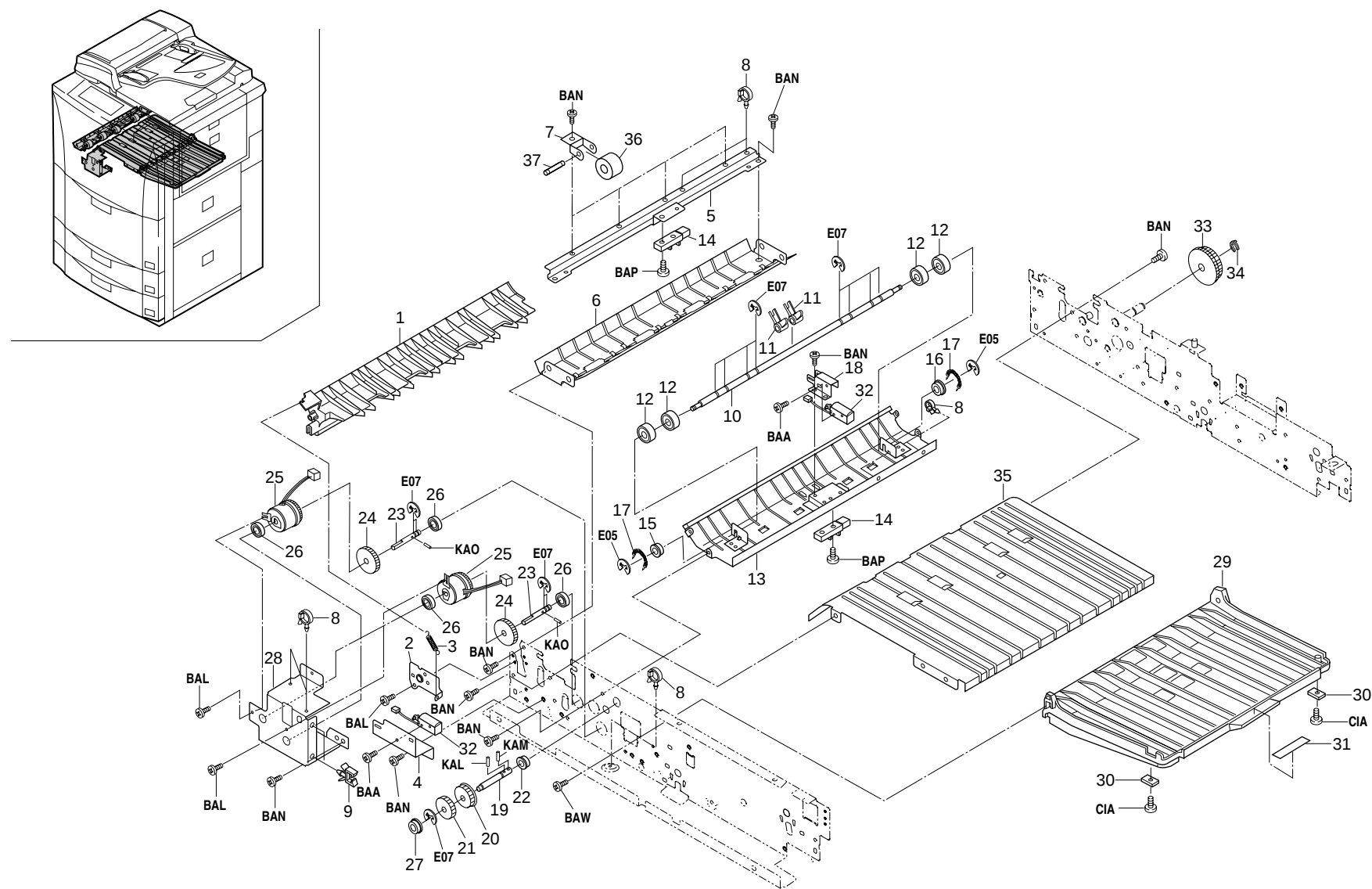
FIG.28 DUPLEX UNIT II
