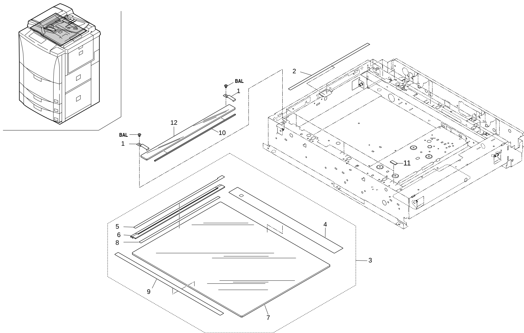
FIG.14 OPTICAL SECTION II
