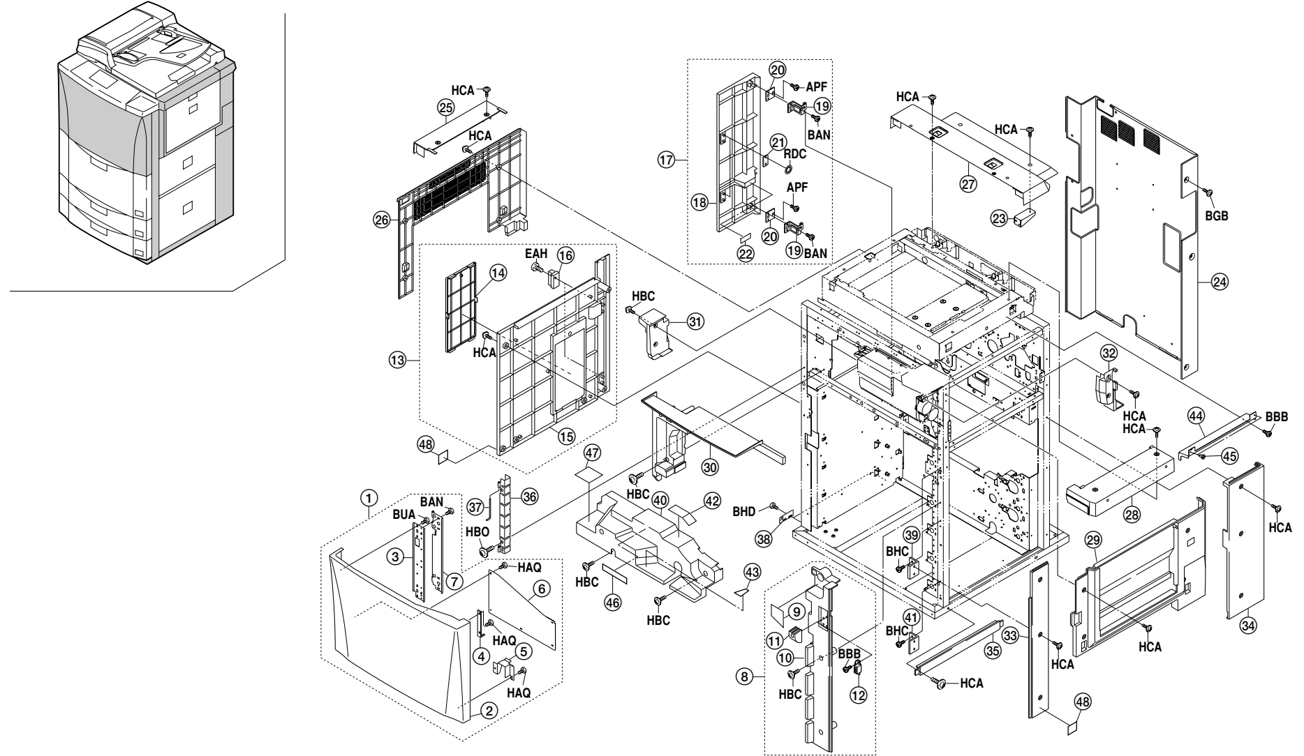
FIG. 1 EXTERIOR COVERS
