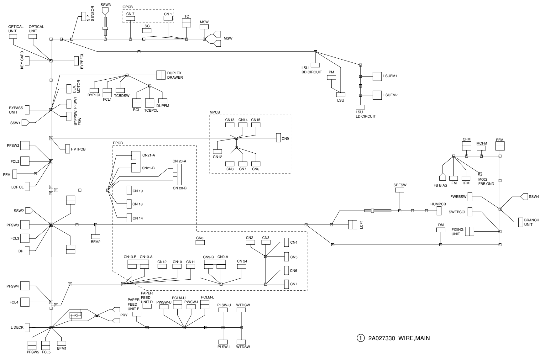
FIG.35 WIRE SECTION II
