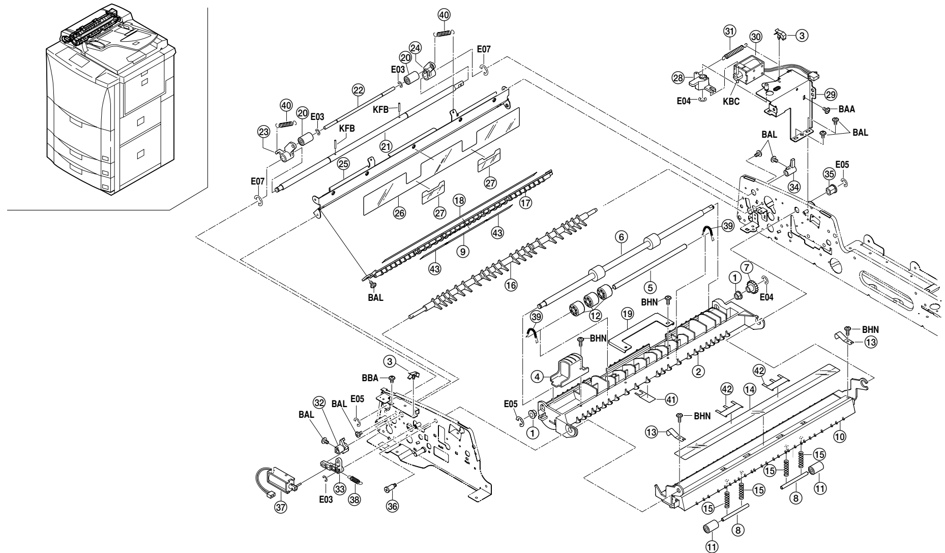
FIG.40 REVERSING SECTION
