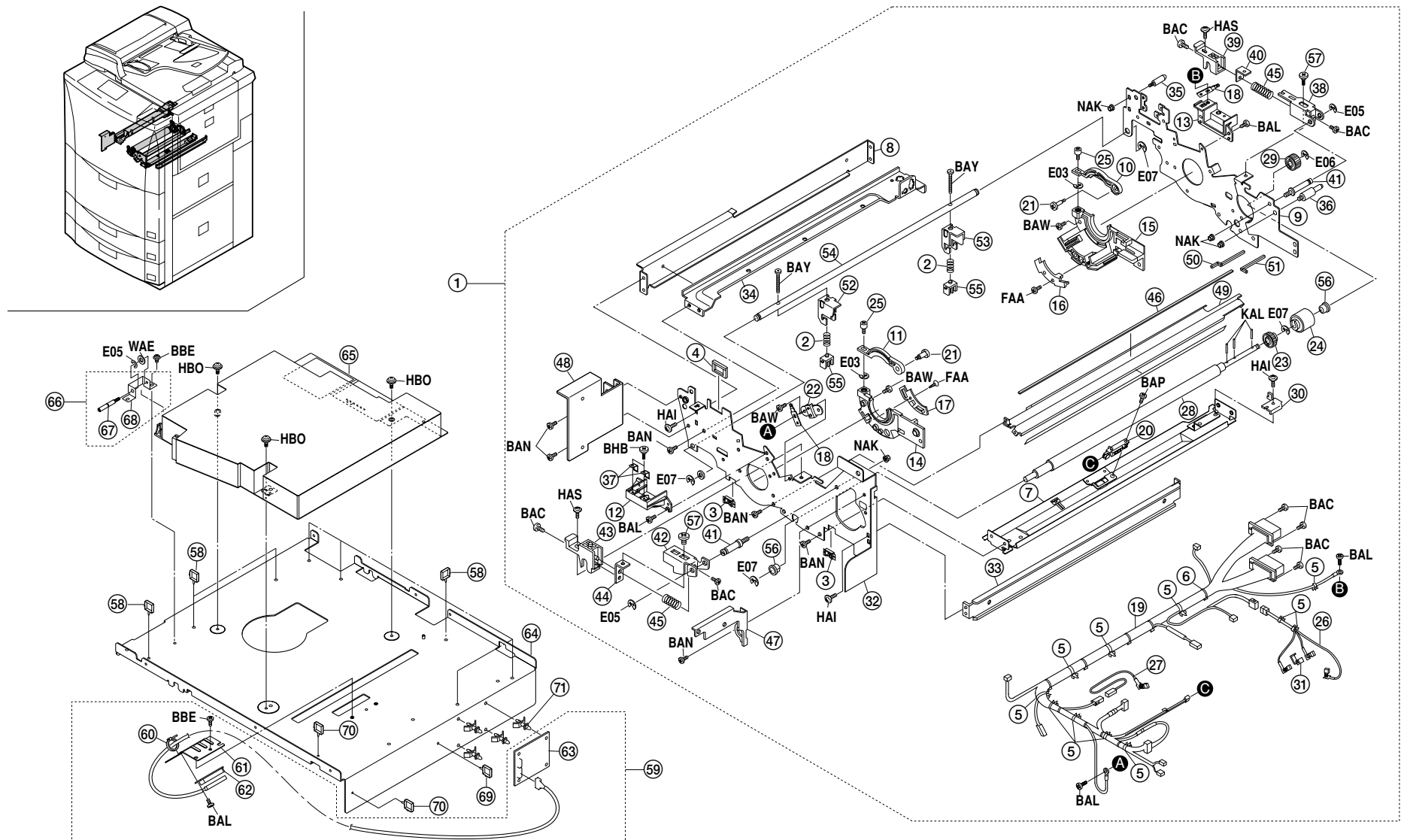
FIG.16 IMAGE FORMATION SECTION II
