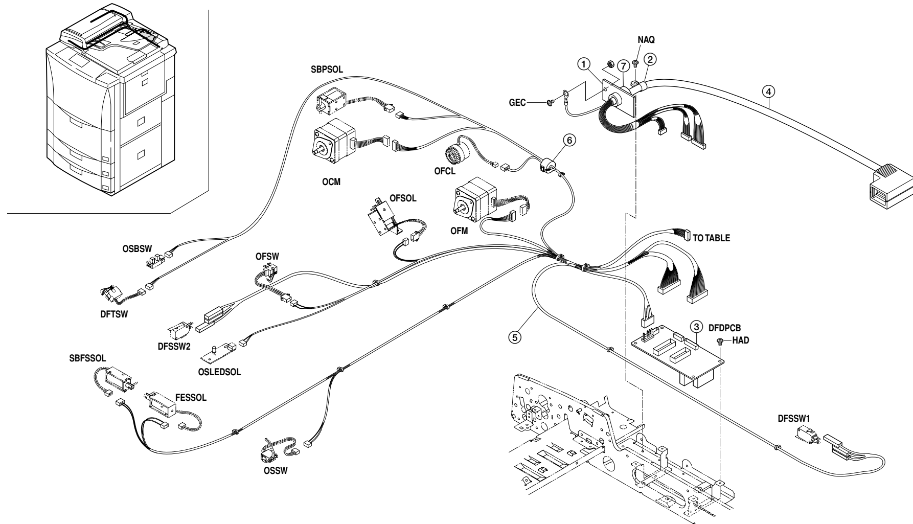
FIG.43 ELECTRICAL COMPONENTS
