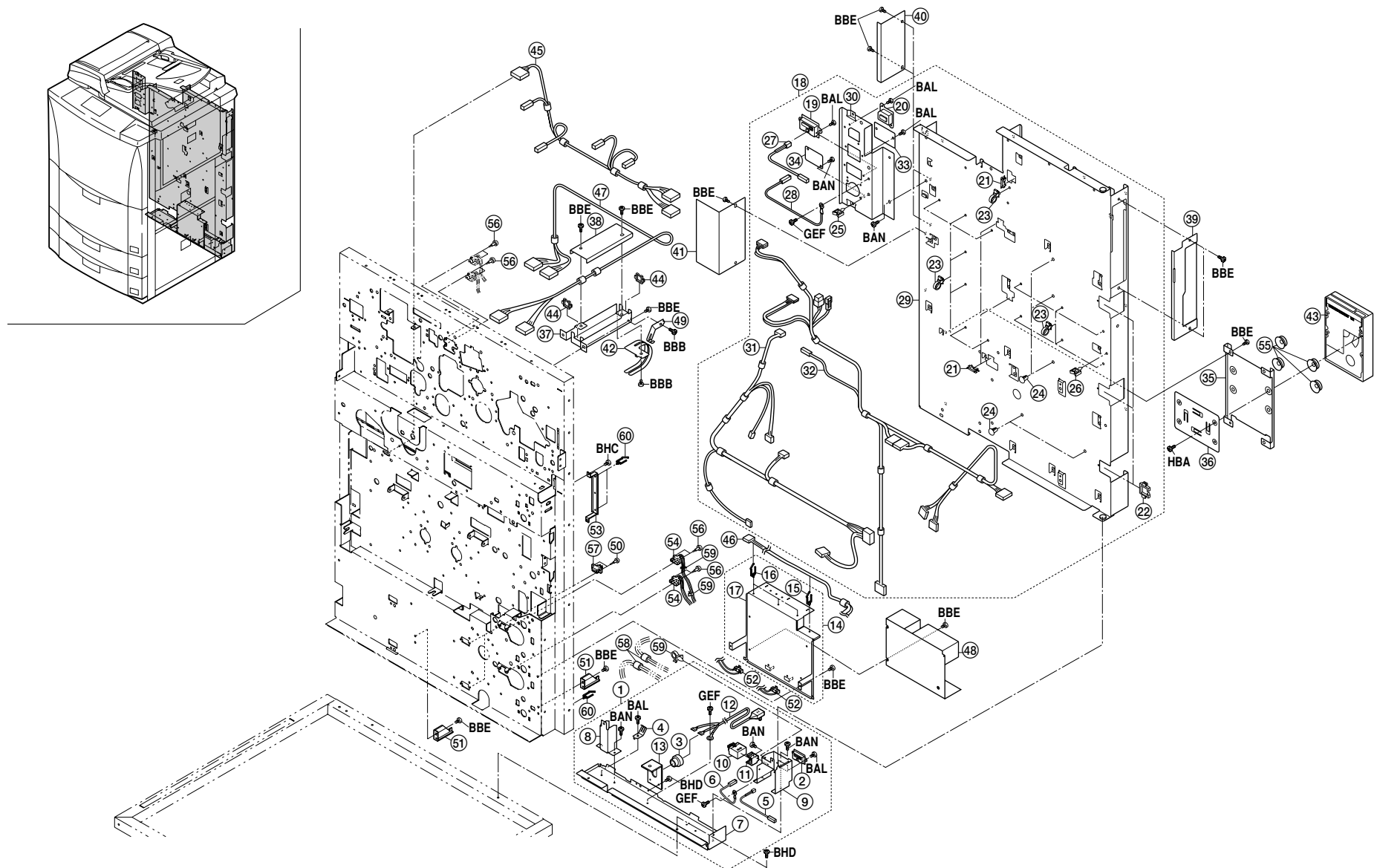
FIG.32 ELECTRICAL COMPONENTS I (120V)
