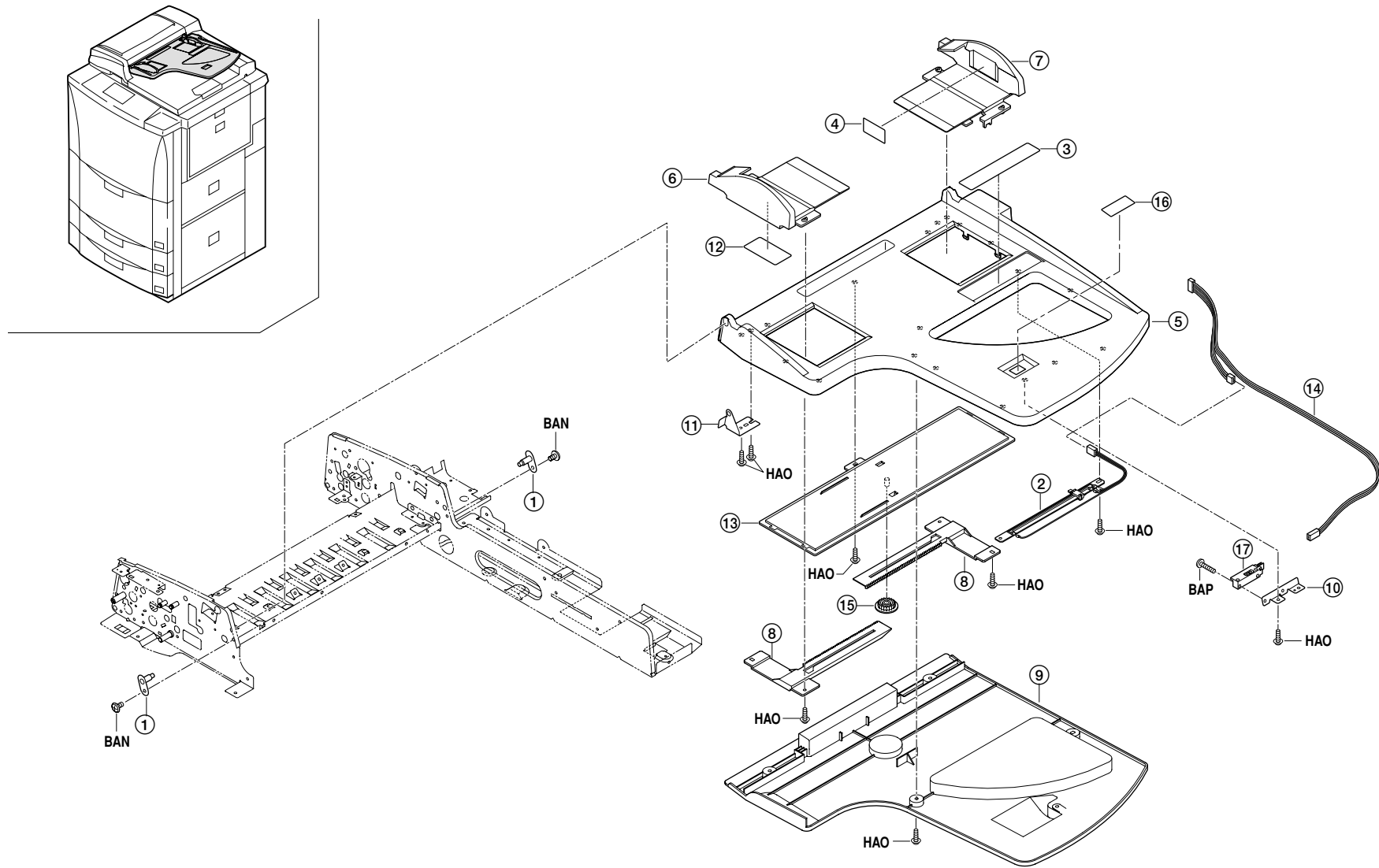
FIG.38 PAPER FEED-IN SECTION
