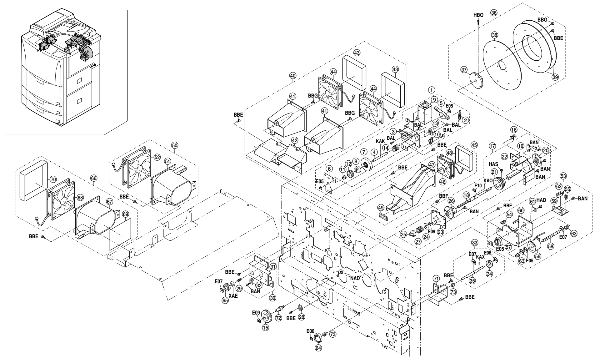
FIG.25 DRIVING, COOLING SECTION II
