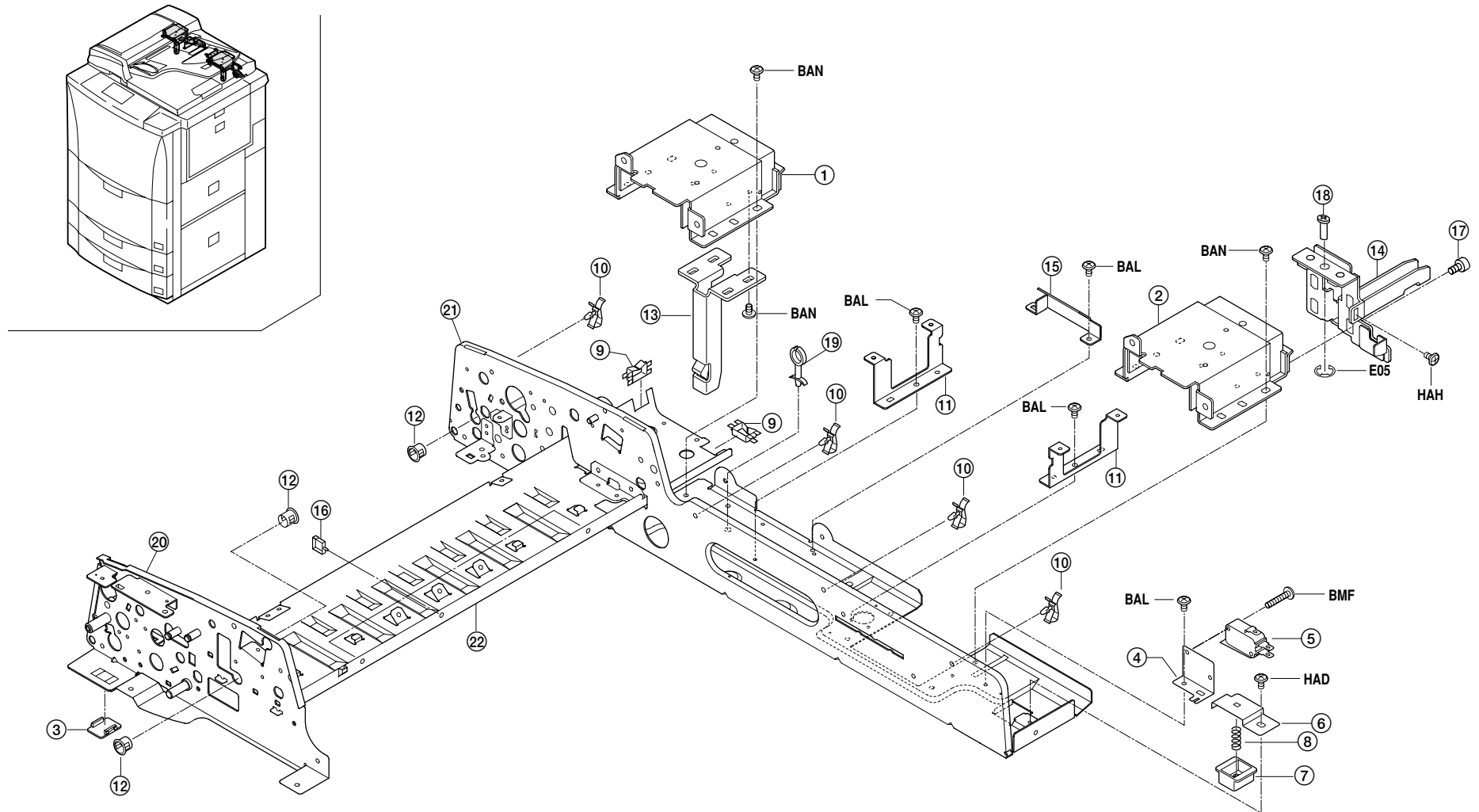
FIG.37 FRAMES
