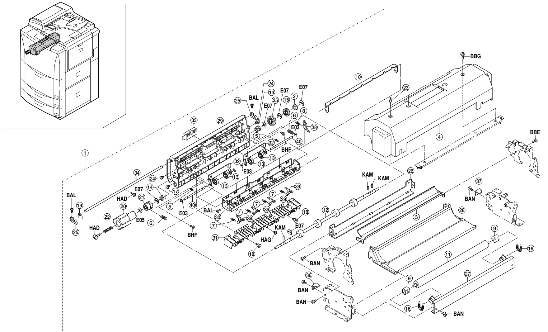
FIG.22 FIXING SECTION I
