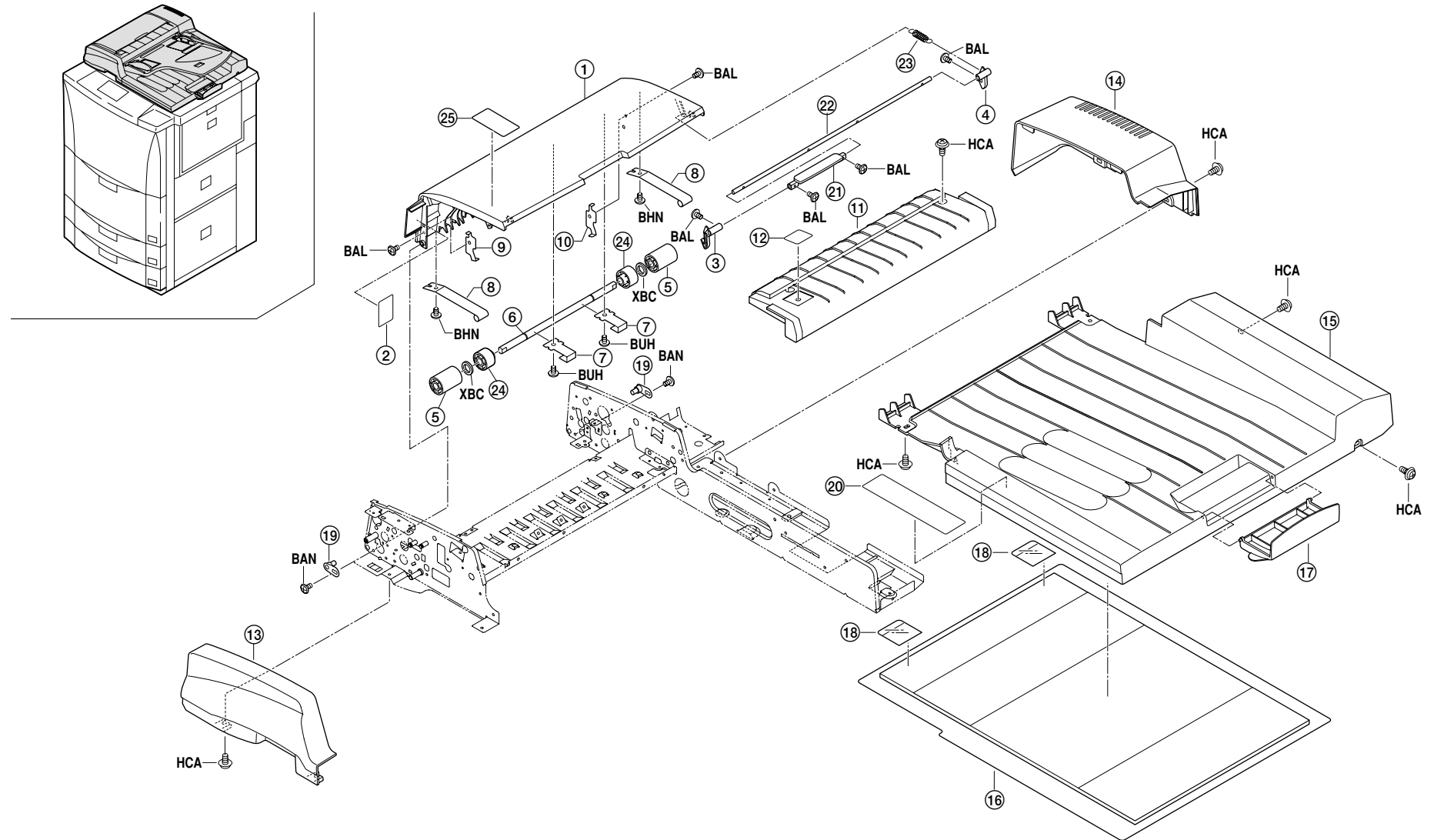
FIG.36 EXTERIOR COVERS
