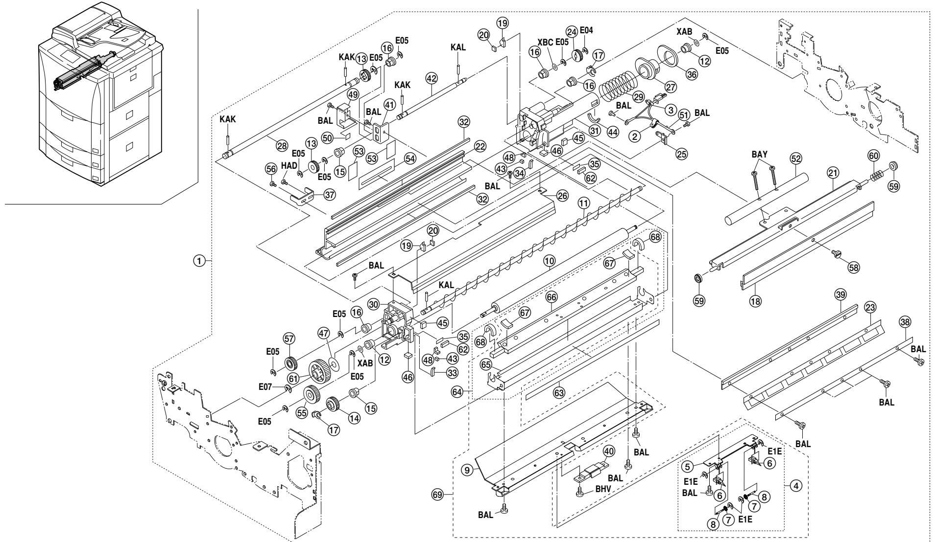
FIG.20 CLEANING SECTION I
