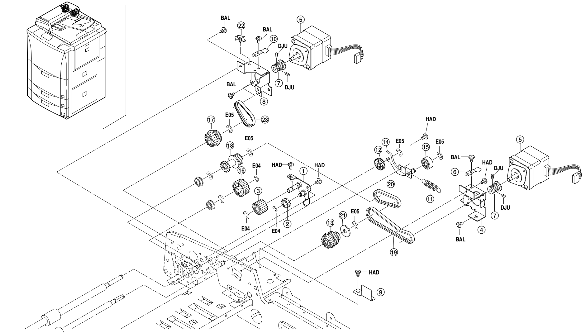
FIG.42 DRIVING SECTION
