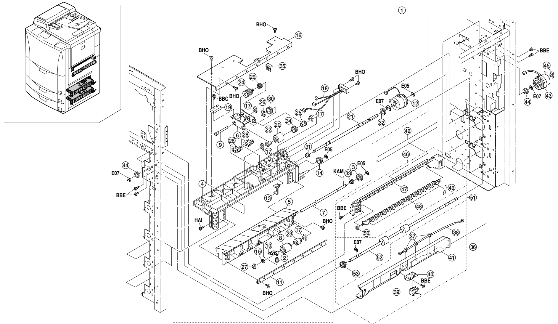
FIG. 8 PAPER FEED-IN SECTION II
