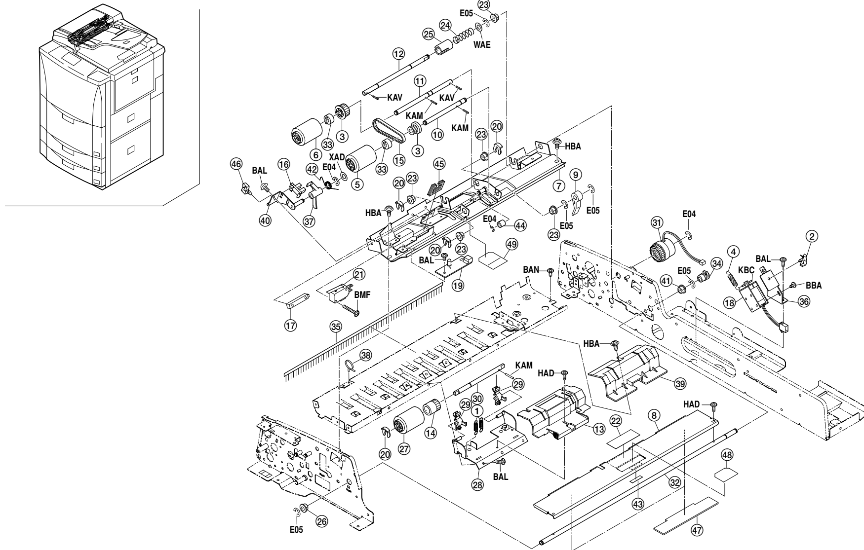
FIG.39 PAPER CONVEYING SECTION
