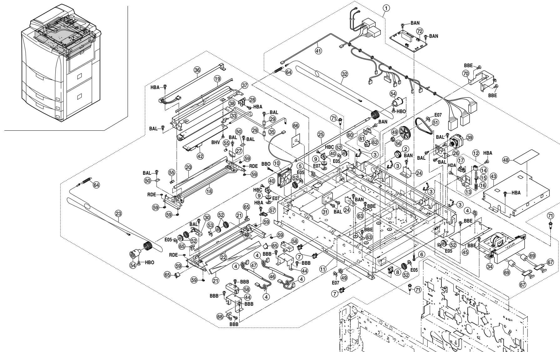
FIG.14 OPTICAL SECTION
