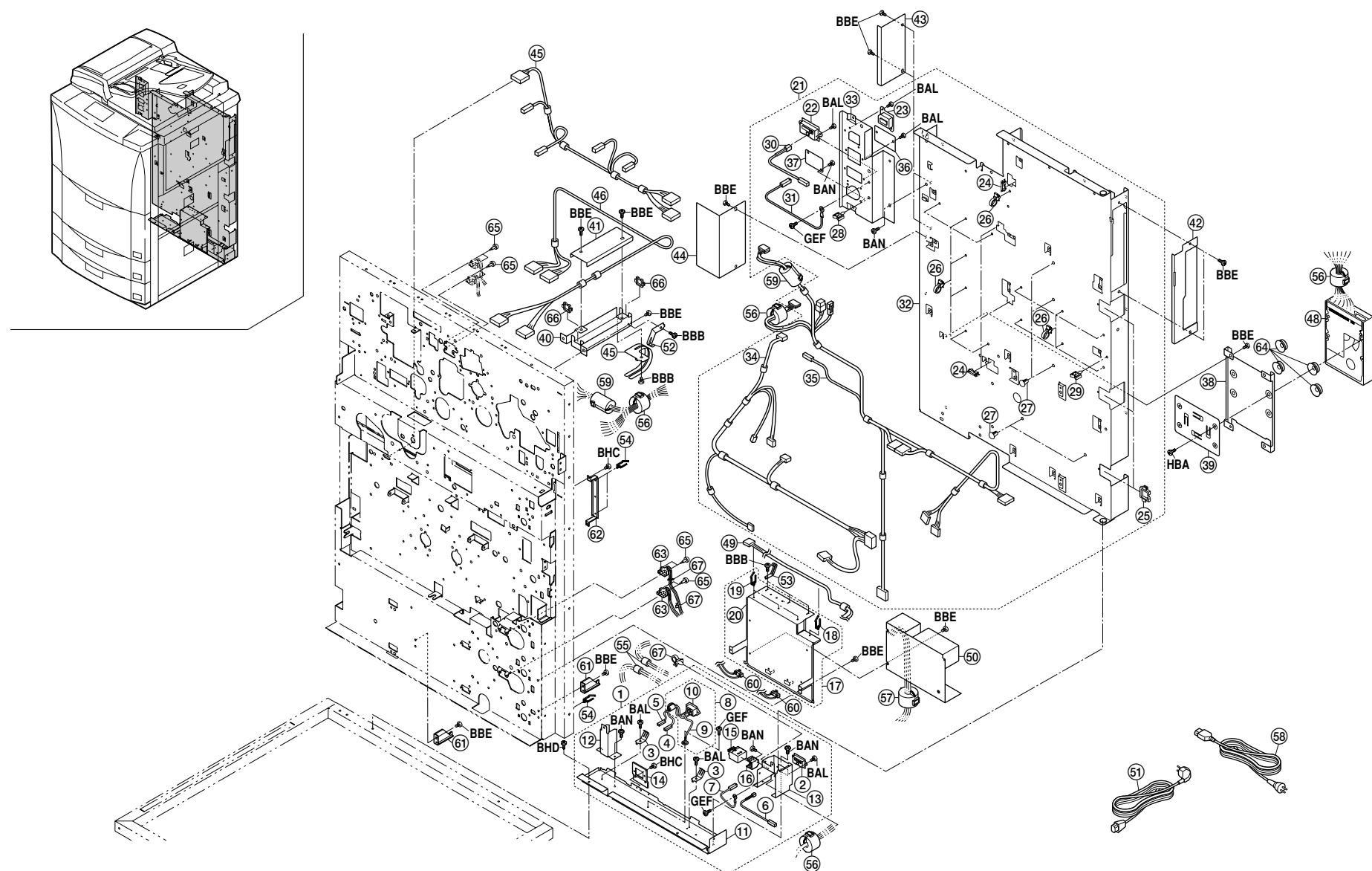
FIG.32 ELECTRICAL COMPONENTS I (230/240V)
