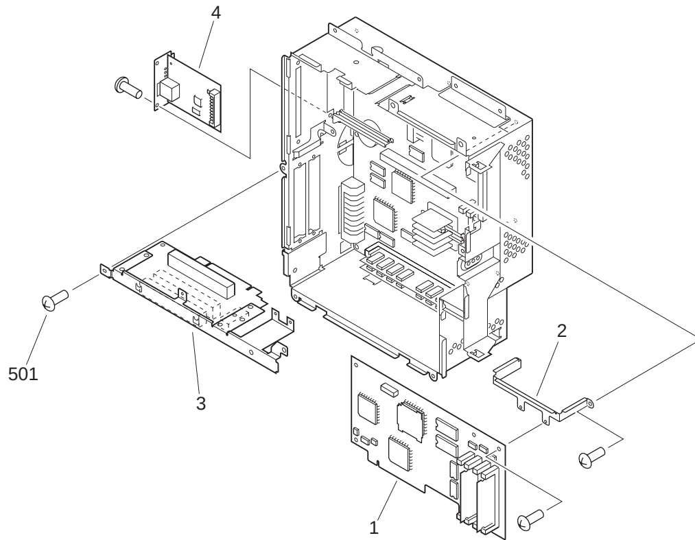
FIGURE U10 NETWORK LIPS PRINTER KIT ASSEMBLY
