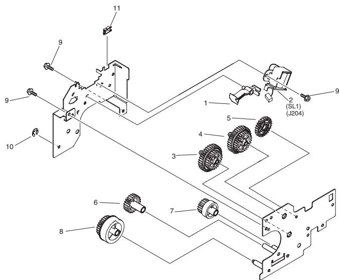
FIGURE 251 REVERSE DRIVE ASSEMBLY
