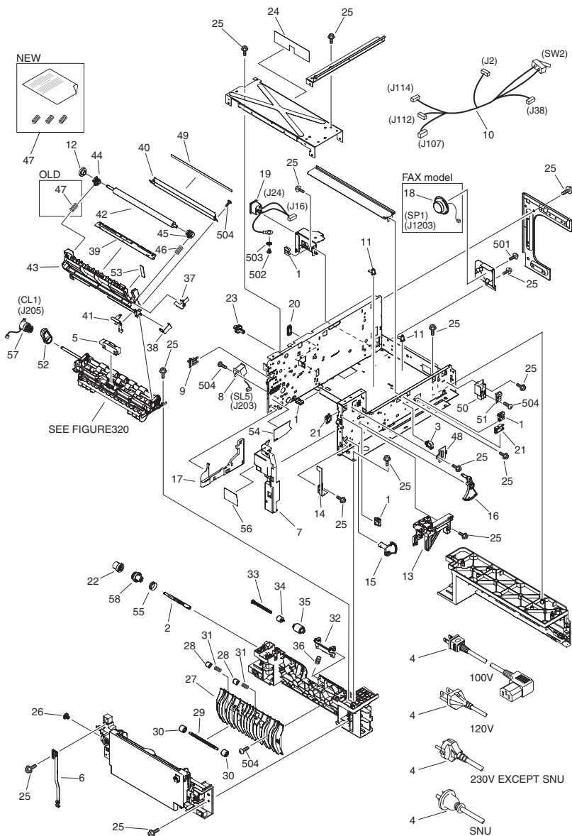
FIGURE 101 Up to SLX/SLY/SNK/SNL/SRS/SRT20000 INTERNAL COMPONENTS 1 (OLD TYPE)
