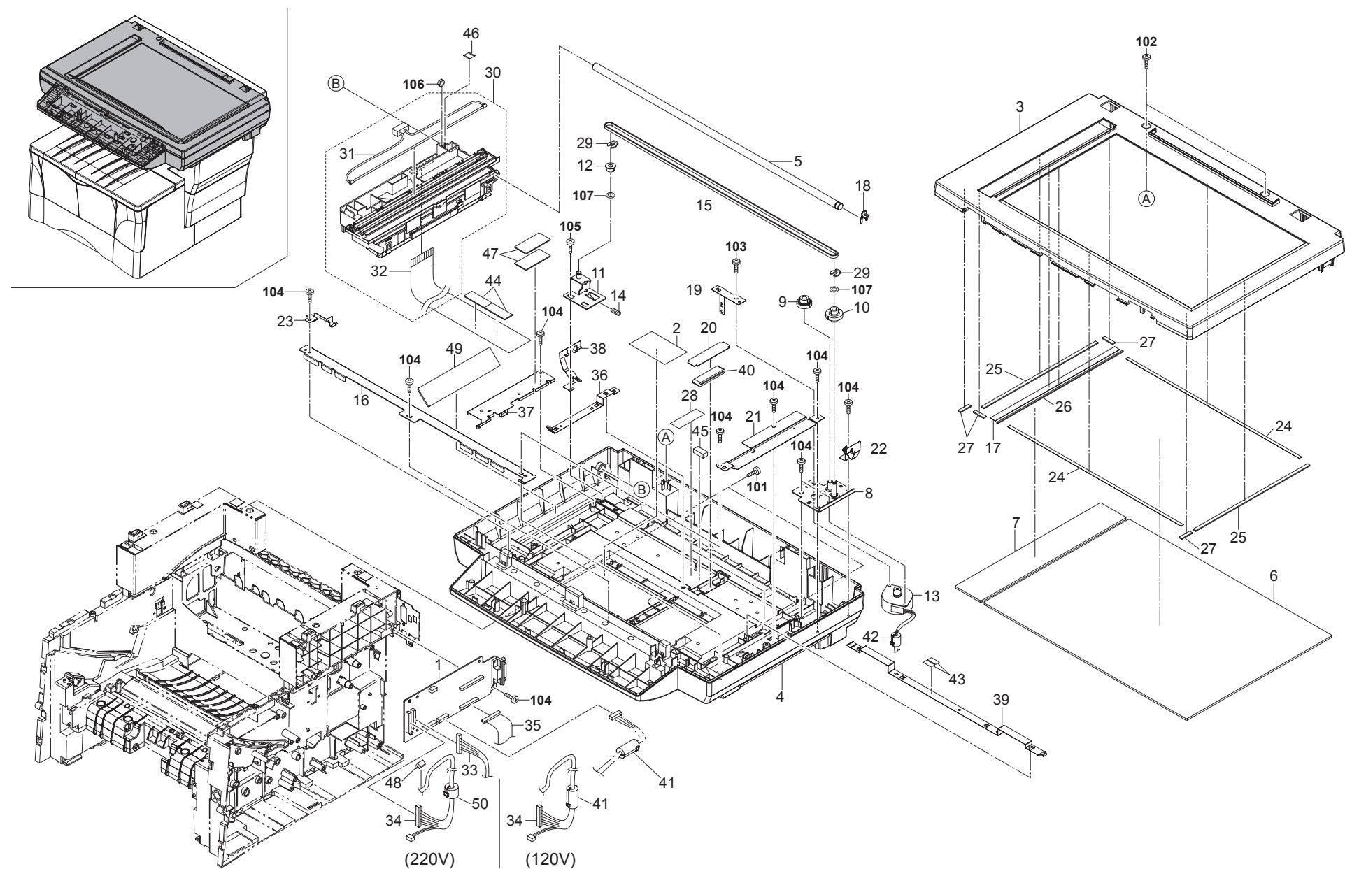
FIG. 8 Optical Section
