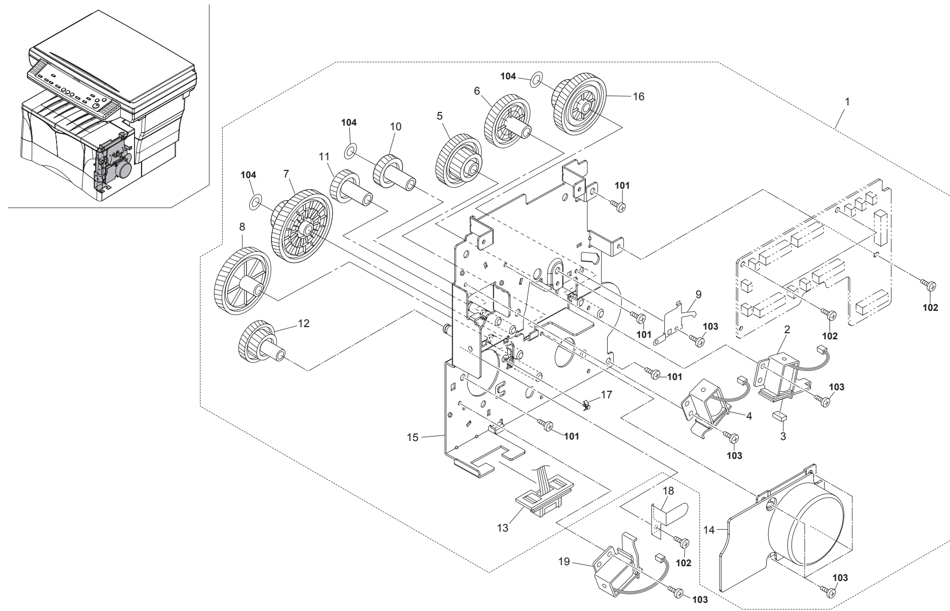
FIG. 4 Driving Section
