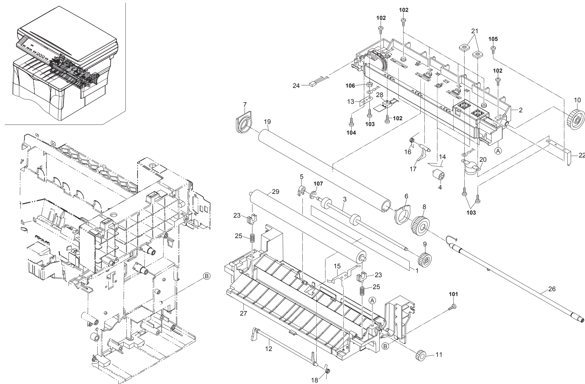
FIG. 6 Fuser Unit
