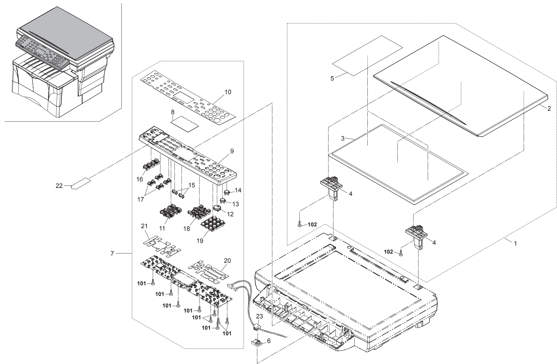
FIG. 9 Operation Unit & Original Holder
