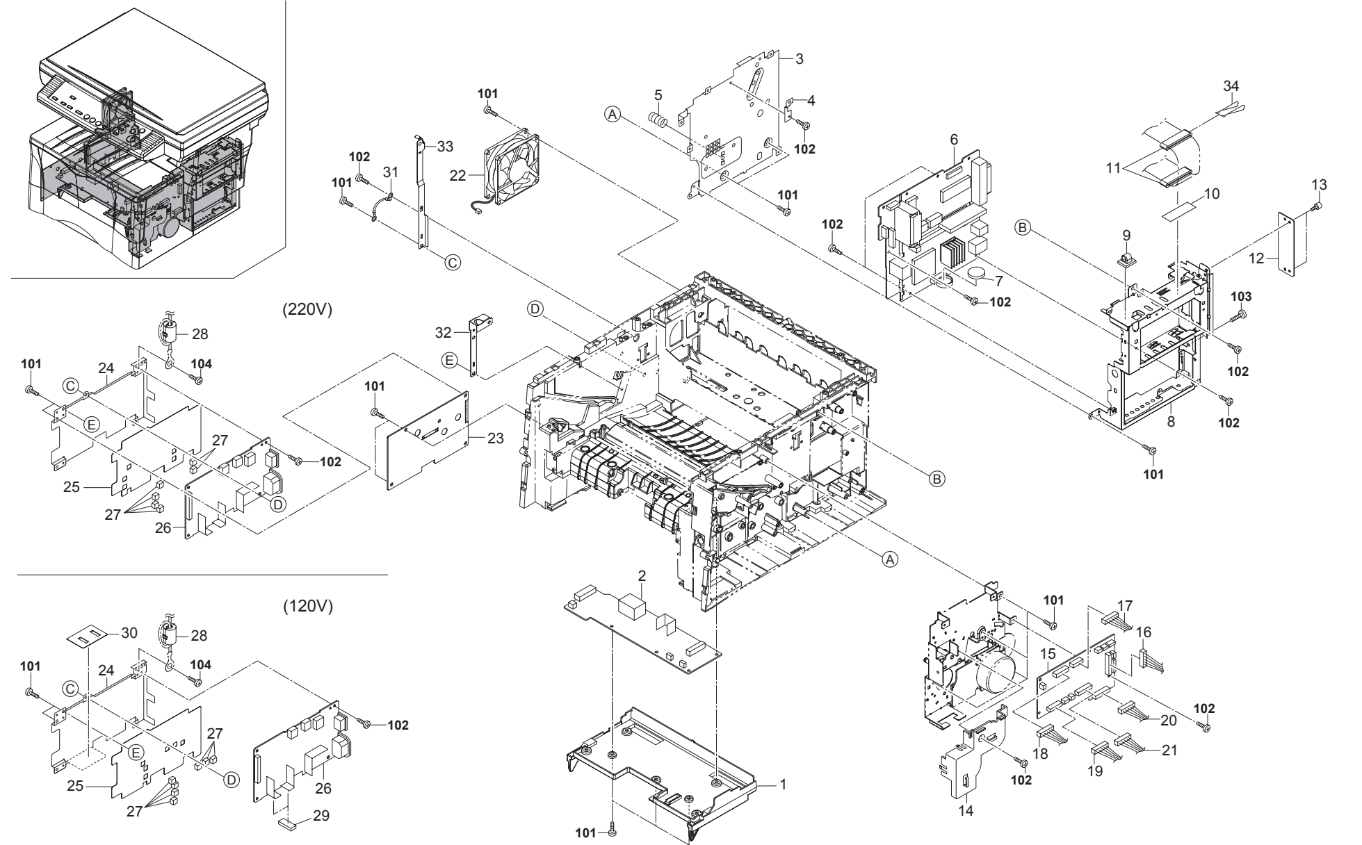
FIG. 10 Electrical Components
