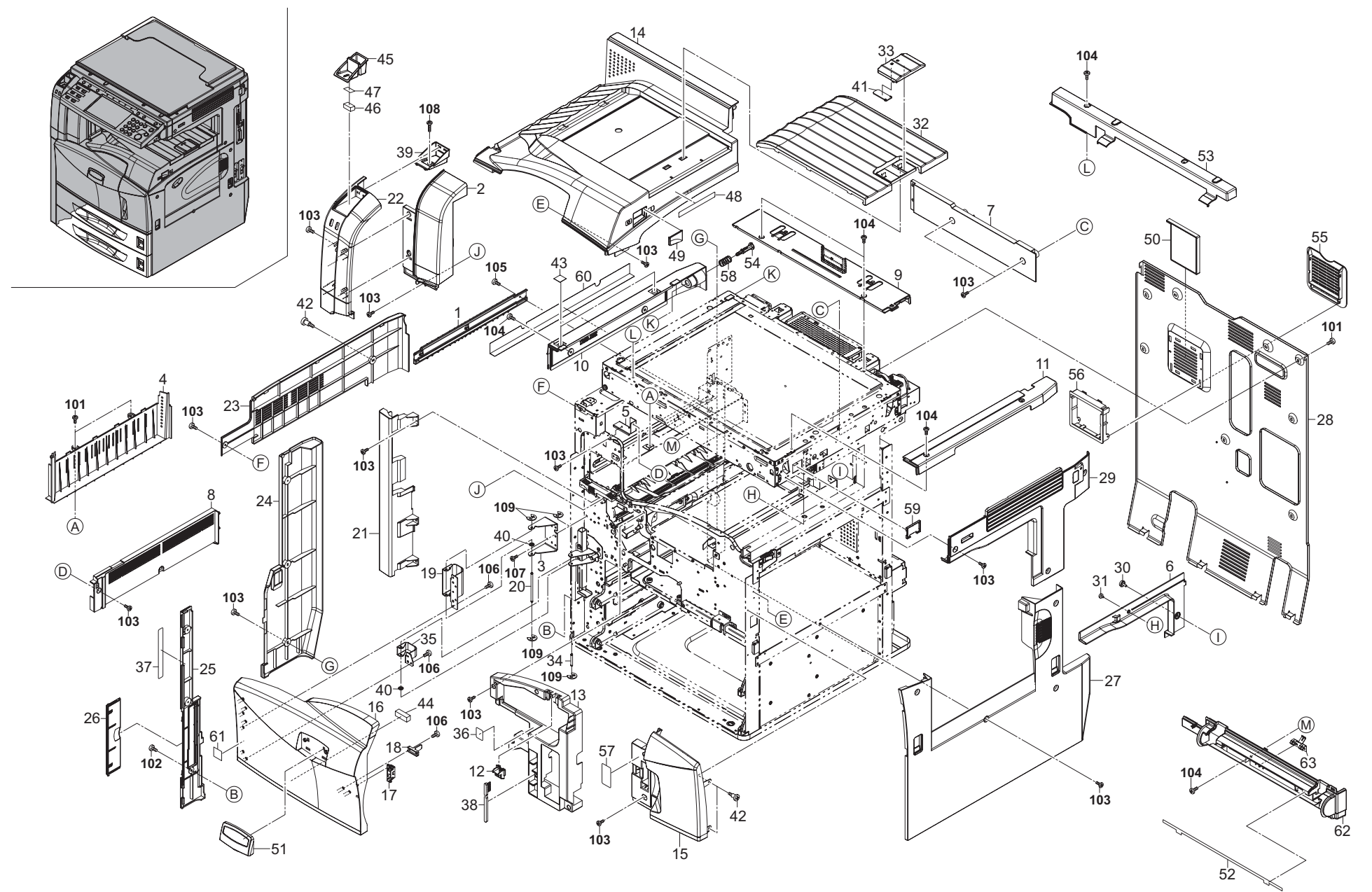
FIG. 1 Covers
