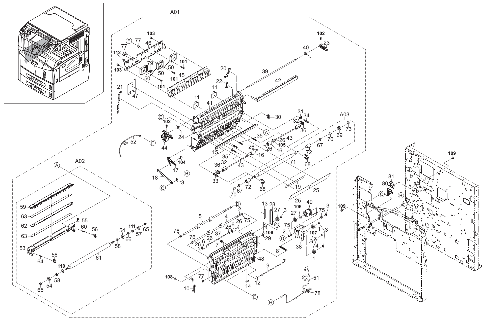
FIG. 7 Paper Conveying
