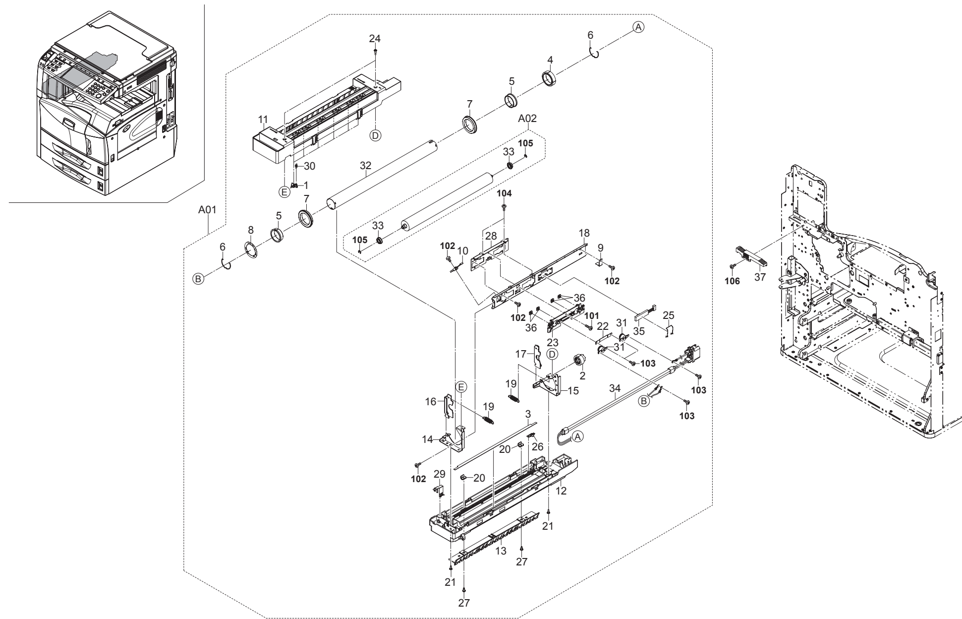
FIG. 15 Fuser Unit
