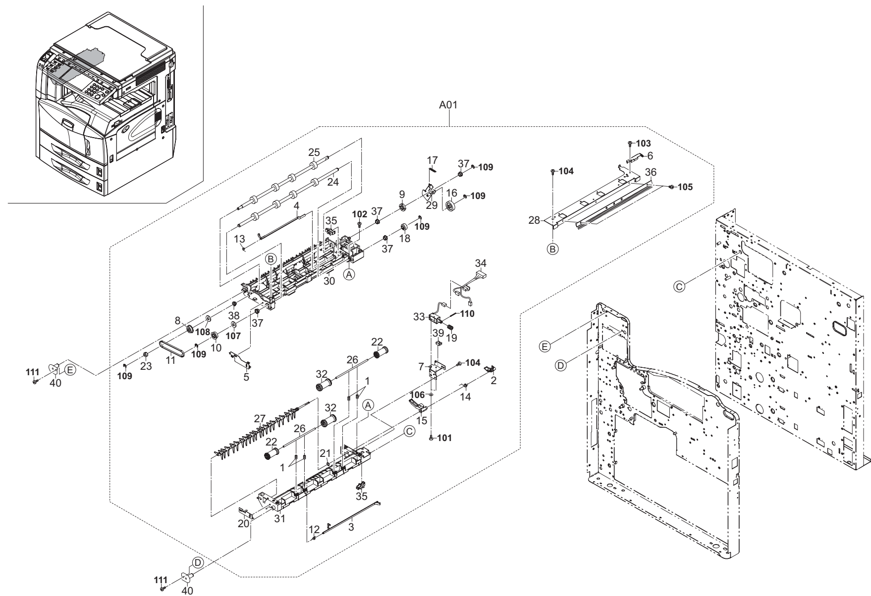
FIG. 8 Paper Exit
