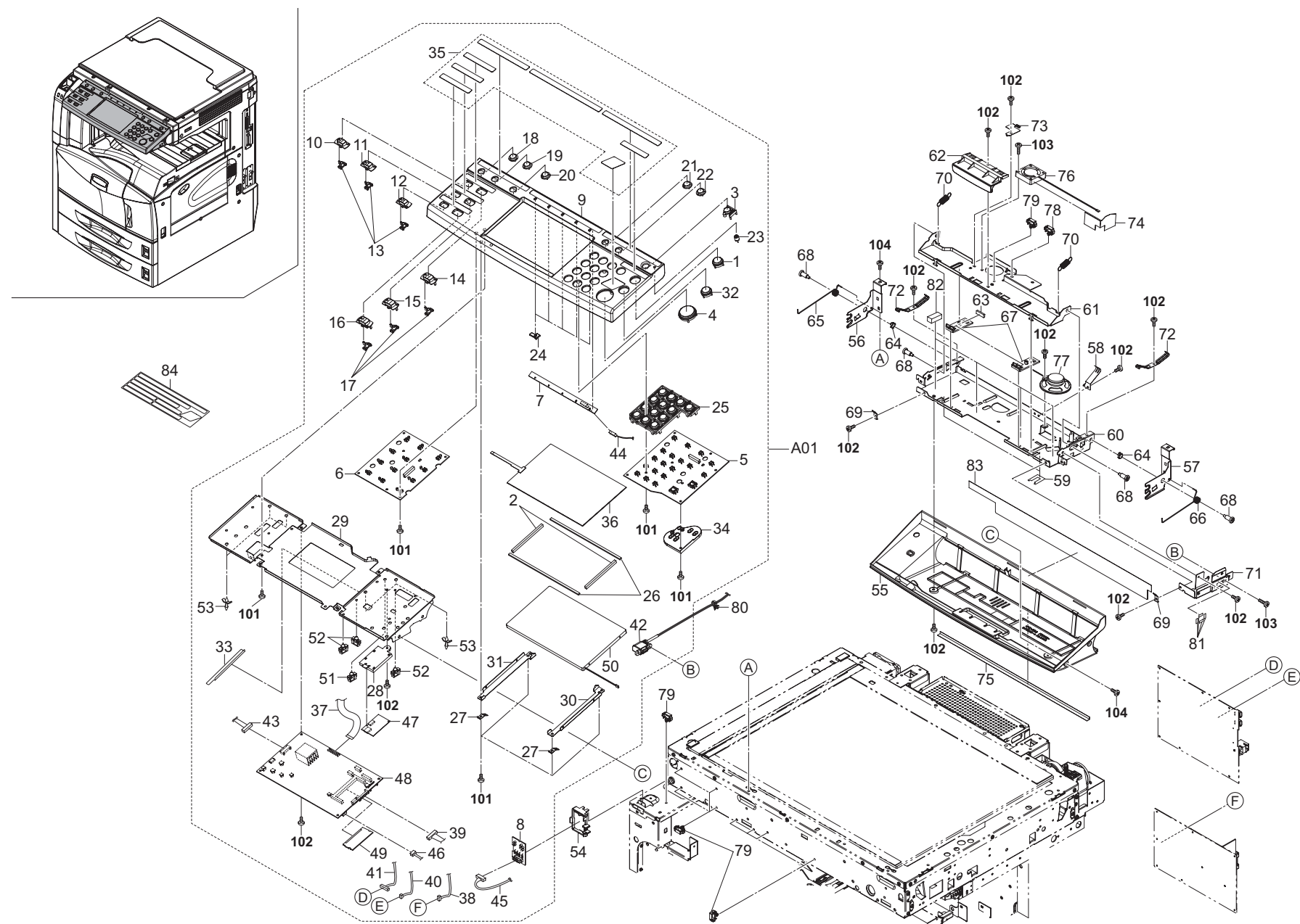
FIG. 21 Operation Unit
