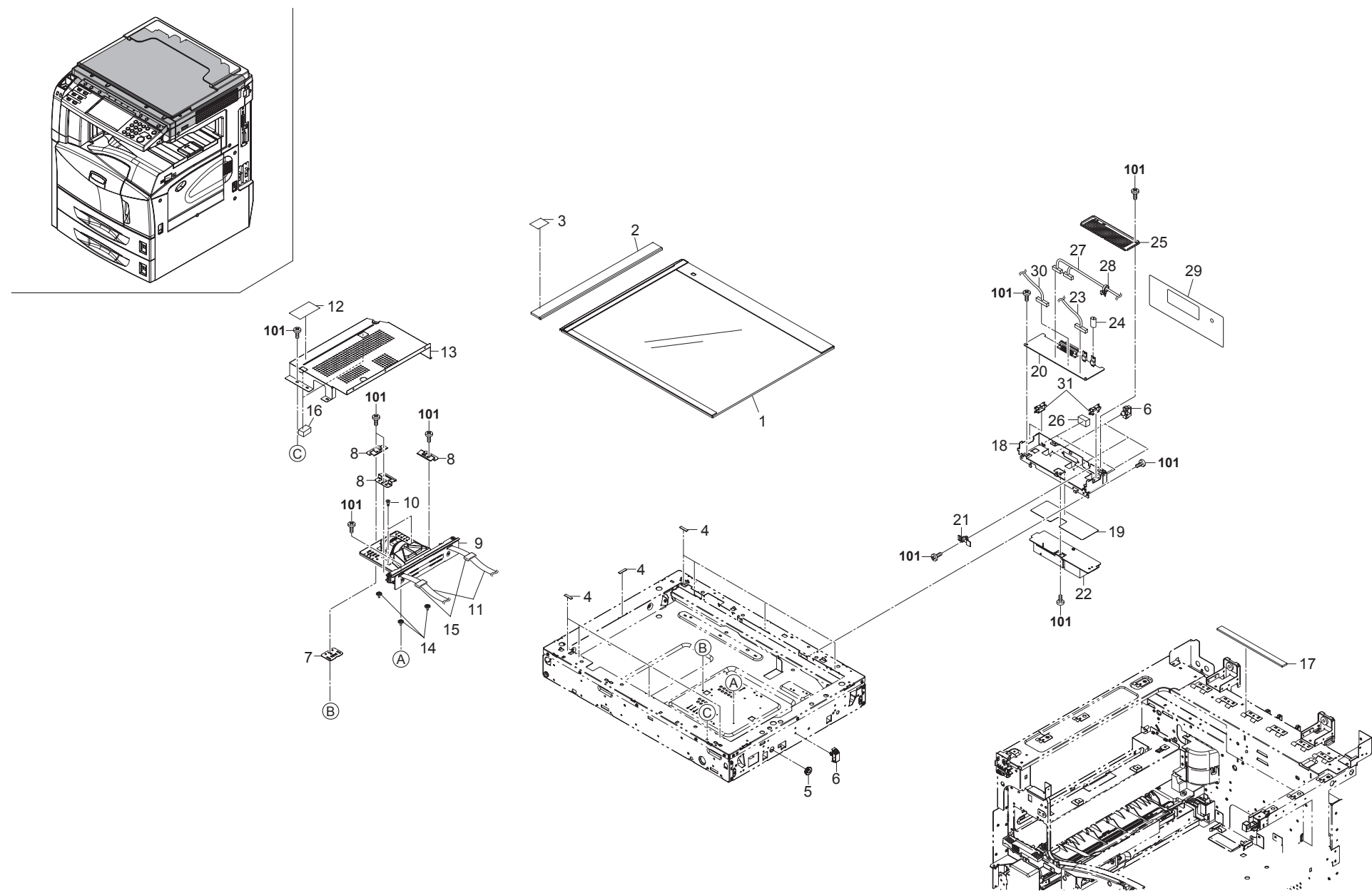
FIG. 10 Scanner Unit II
