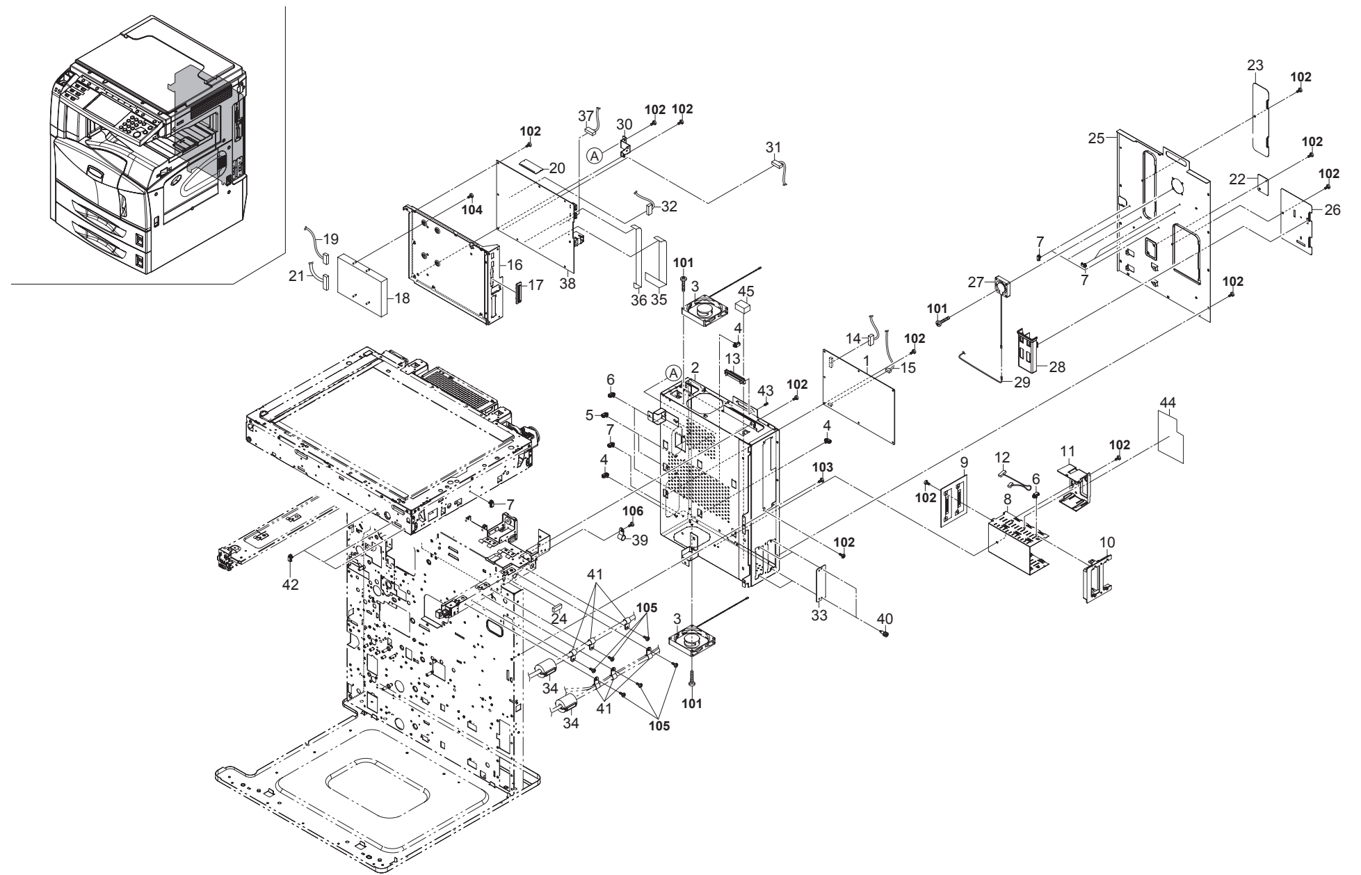
FIG. 20 Electrical Components II
