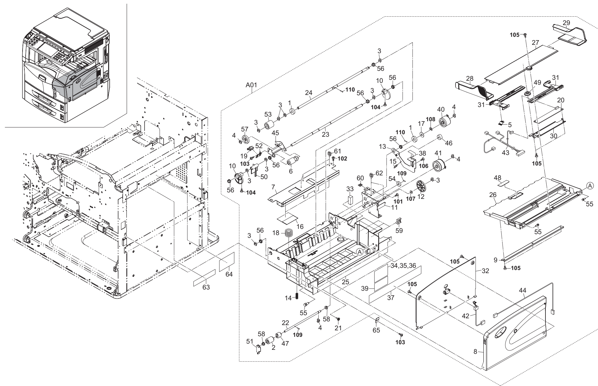
FIG. 11 Bypass Unit
