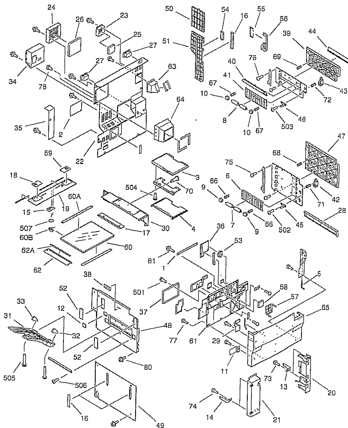
FIGURE 100 EXTERNAL COVERS, PANELS, ETC. 外装カバー
