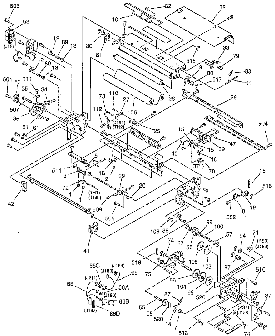
FIGURE 810 FIXING ASSEMBLY(2/2) 定着器(2/2)
