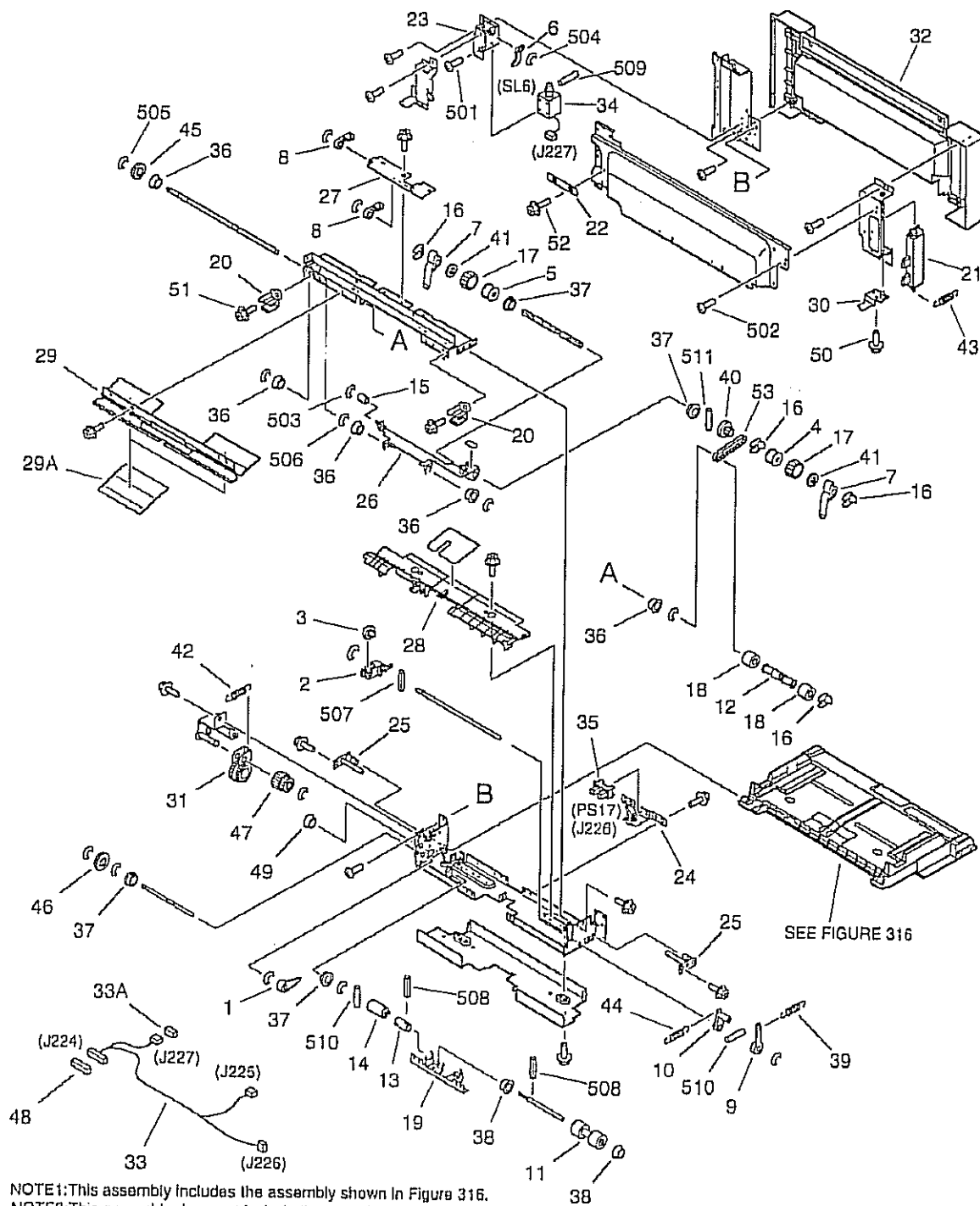
FIGURE 315 MULTI FEED ASSEMBLY
