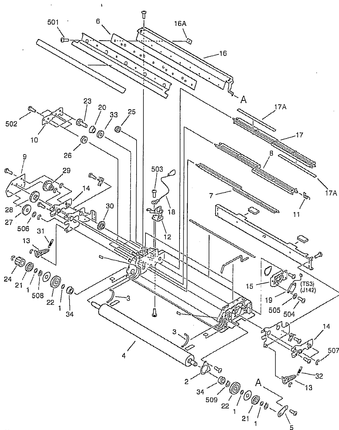
FIGURE 640 DEVELOPING ASSEMBLY 現像器
