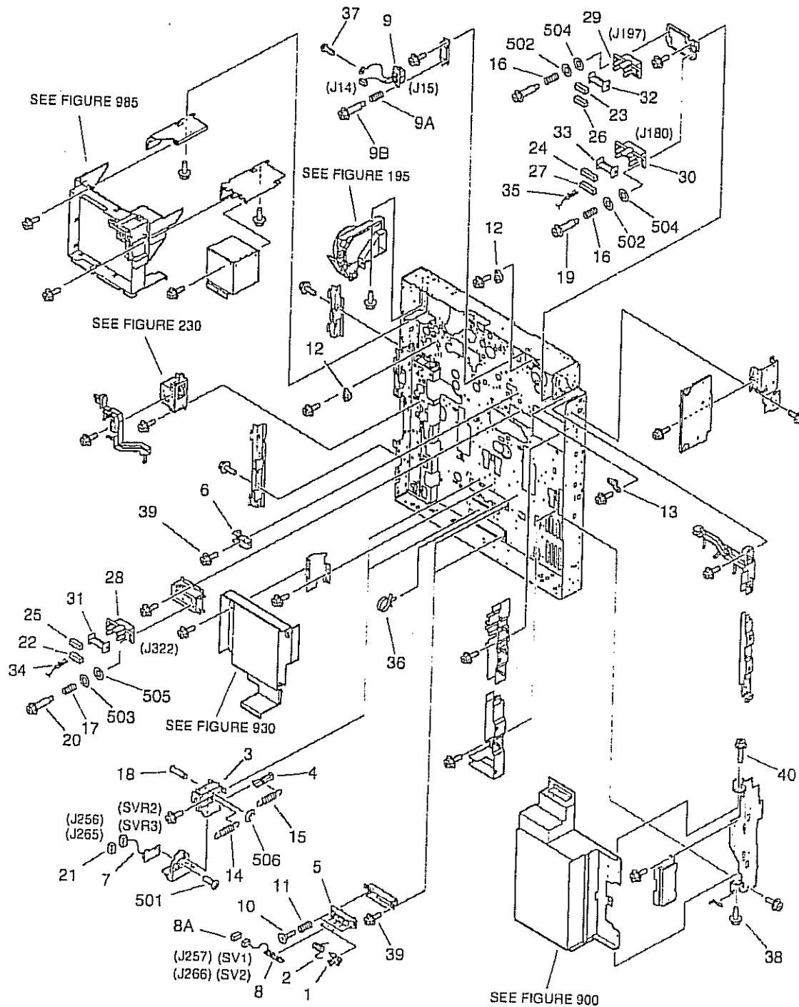
FIGURE 107 MACHINE REAR PLATE 2 本体後側板 (2)
