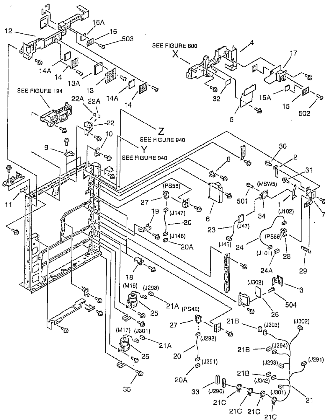
FIGURE 101 MACHINE FRONT PLATE 本体前側板
