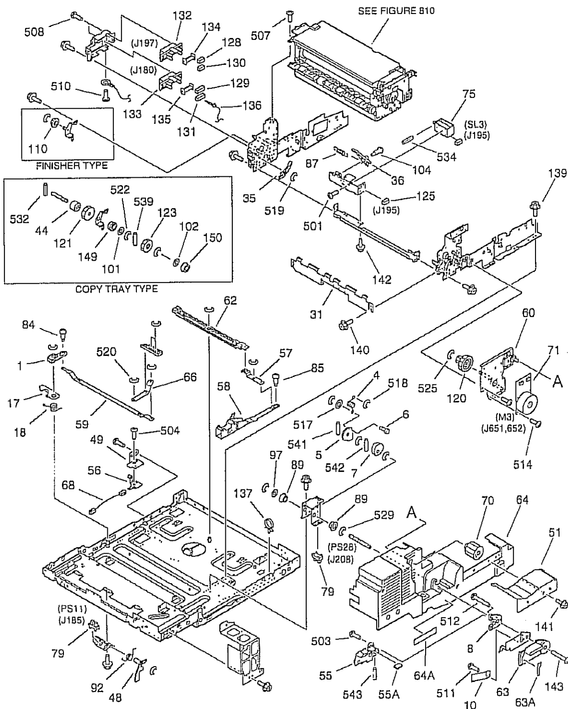
FIGURE 320 FIXING/FEEDER FRAME ASSEMBLY(1/3) 定着/搬送基台部(1/3)
