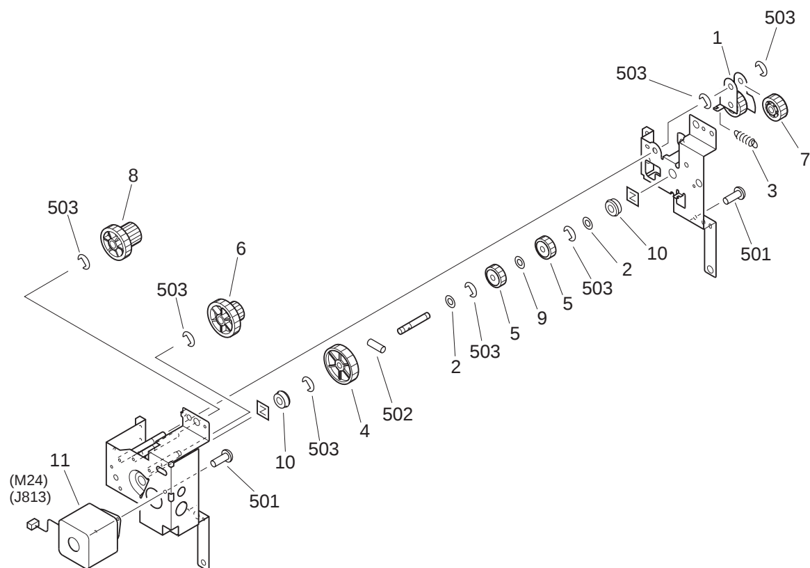
FIGURE 280 FIXING DRIVE ASSEMBLY 定着駆動部
