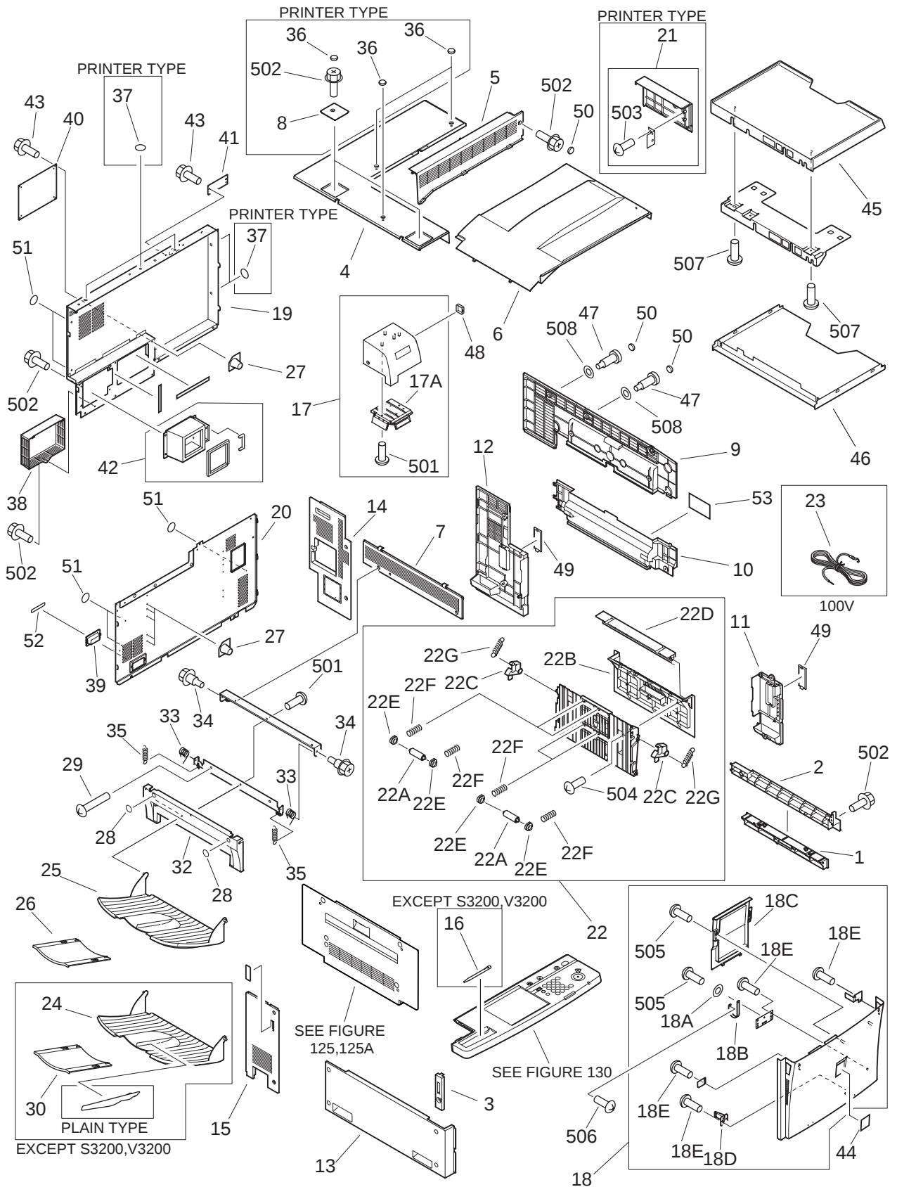
FIGURE 100 EXTERNAL COVERS, PANELS, ETC. 外装カバー
