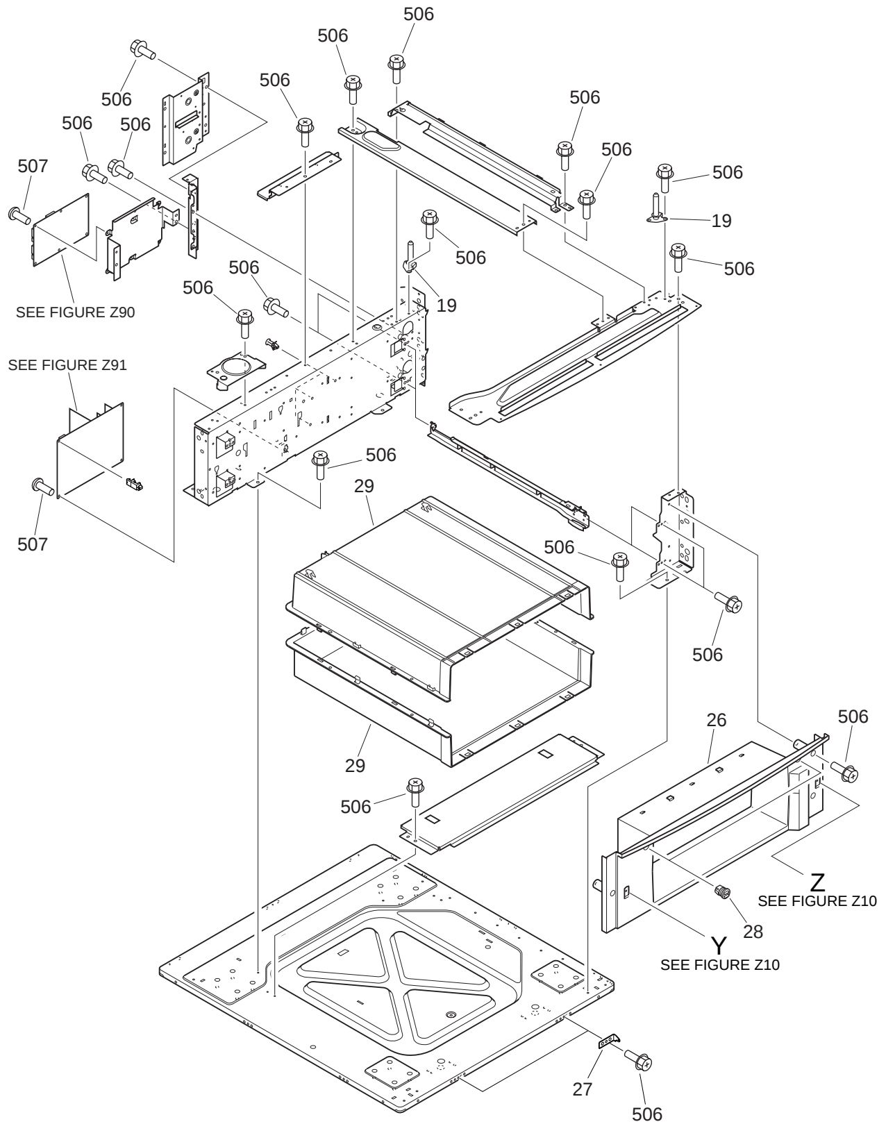
FIGURE Z11 INTERNAL COMPONENTS (2/2) 本体機械内部 (2/2)
