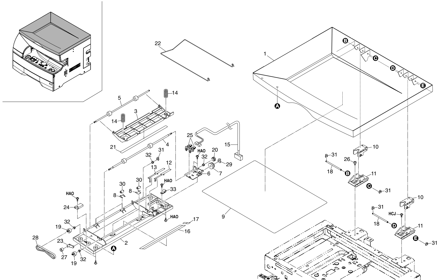
FIG. 5 DOCUMENT FEEDER (1510)
