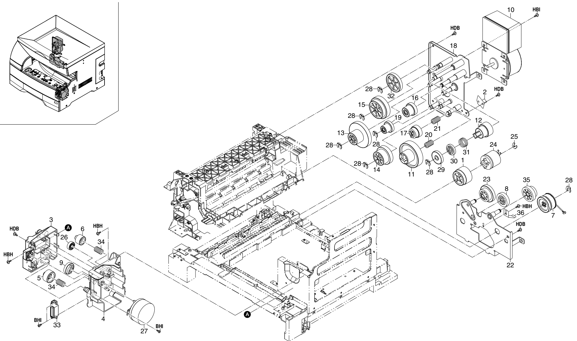
FIG. 13 DRIVING SECTION
