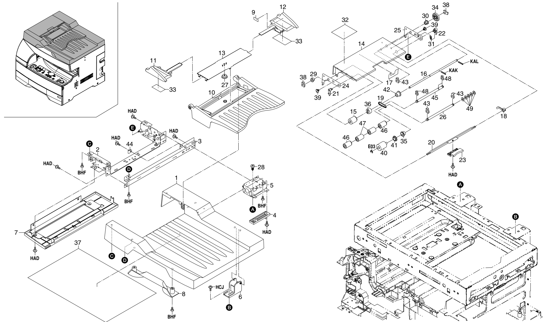
FIG. 6 AUTO DOCUMENT FEEDER I (1810)
