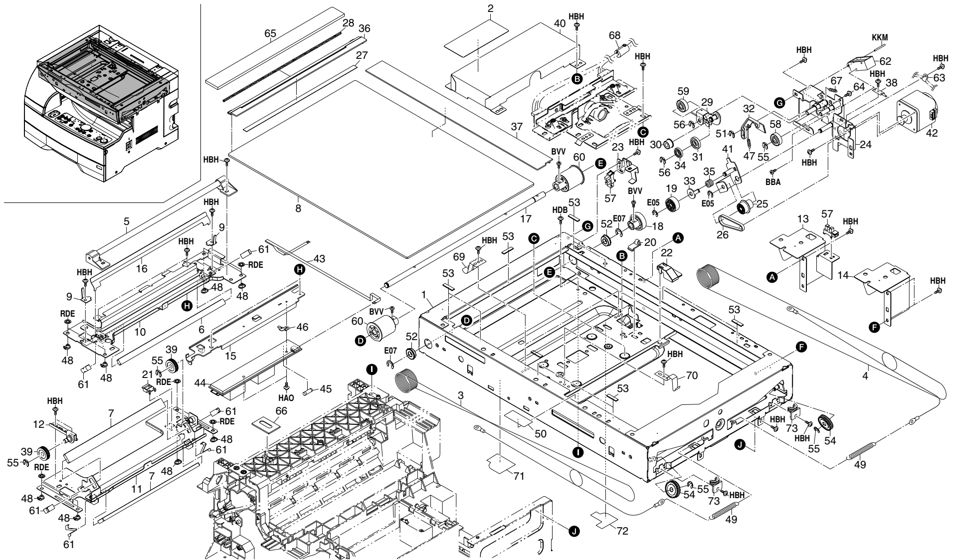
FIG. 8 OPTICAL SECTION
