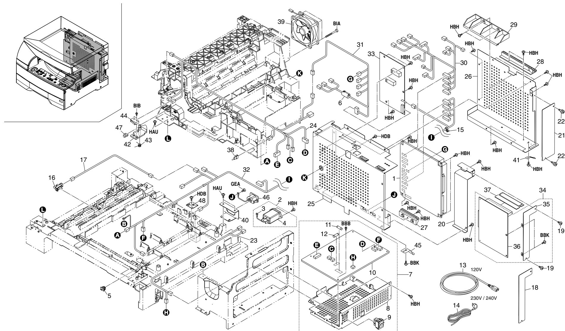
FIG. 14 ELECTRICAL COMPONENTS
