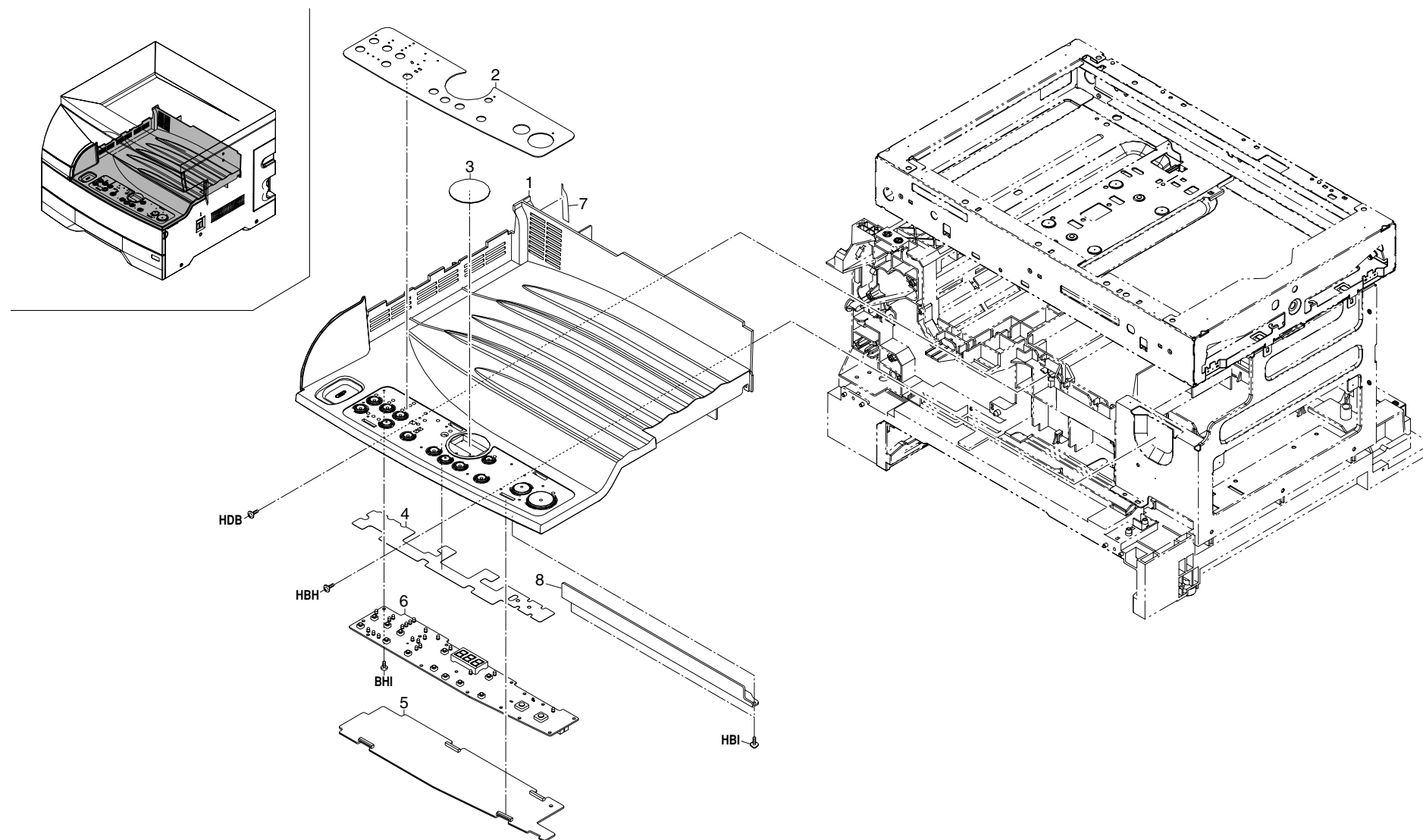
FIG. 15 OPERATION UNIT
