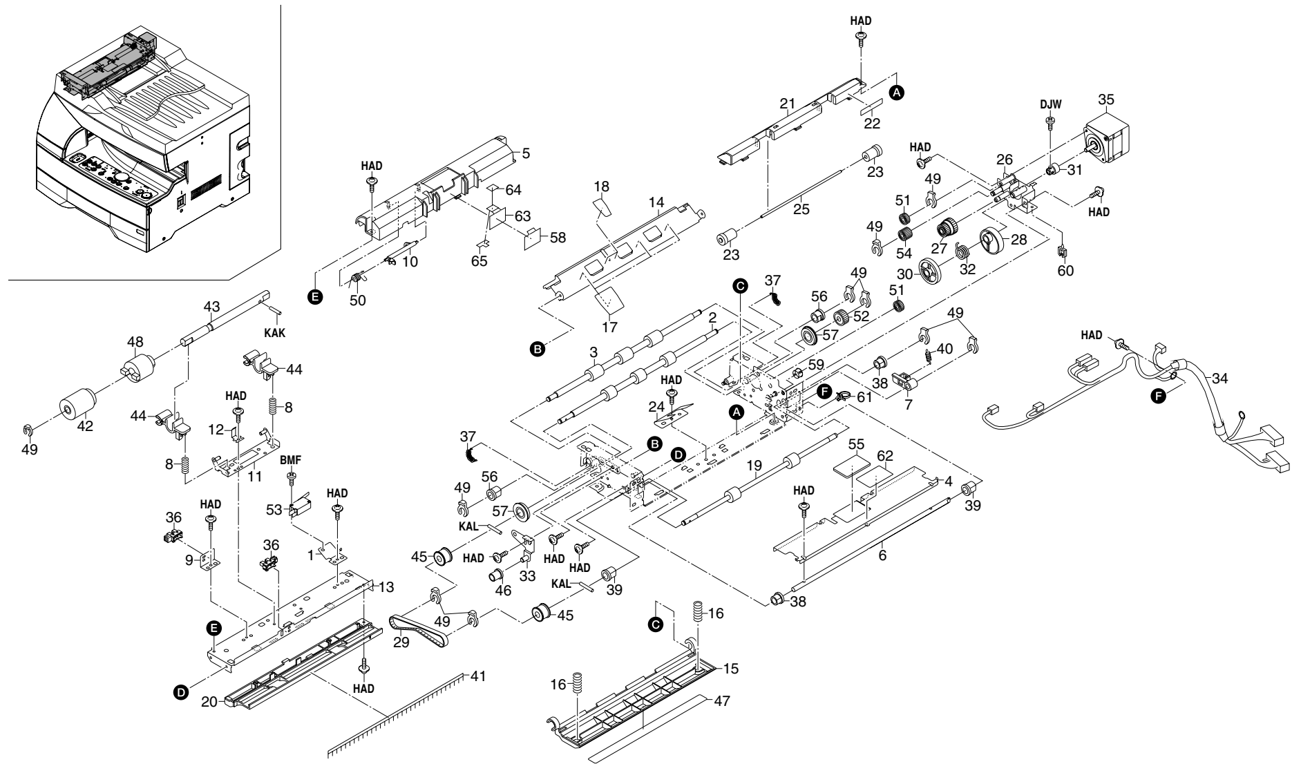
FIG. 7 AUTO DOCUMENT FEEDER II (1810)
