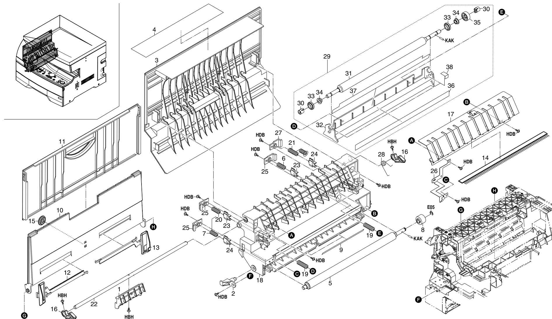
FIG. 4 CONVEYING SECTION
