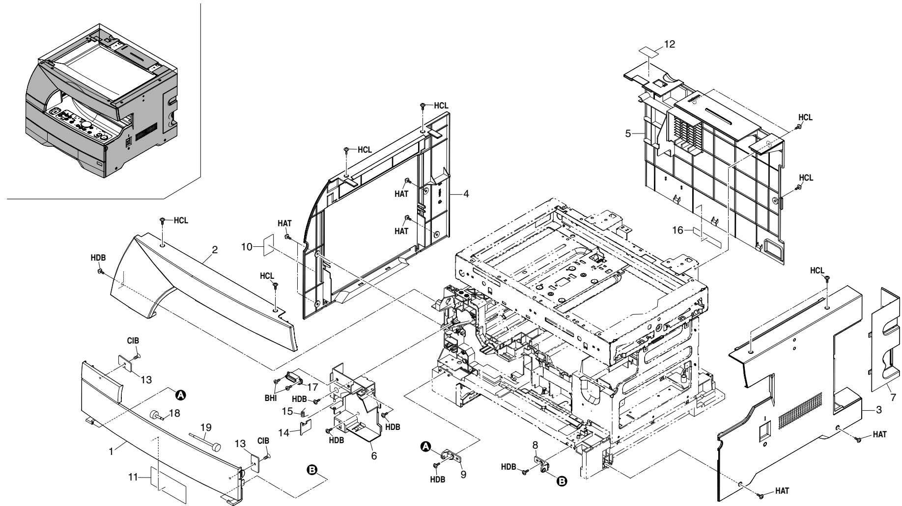
FIG. 1 EXTERIOR COVERS
