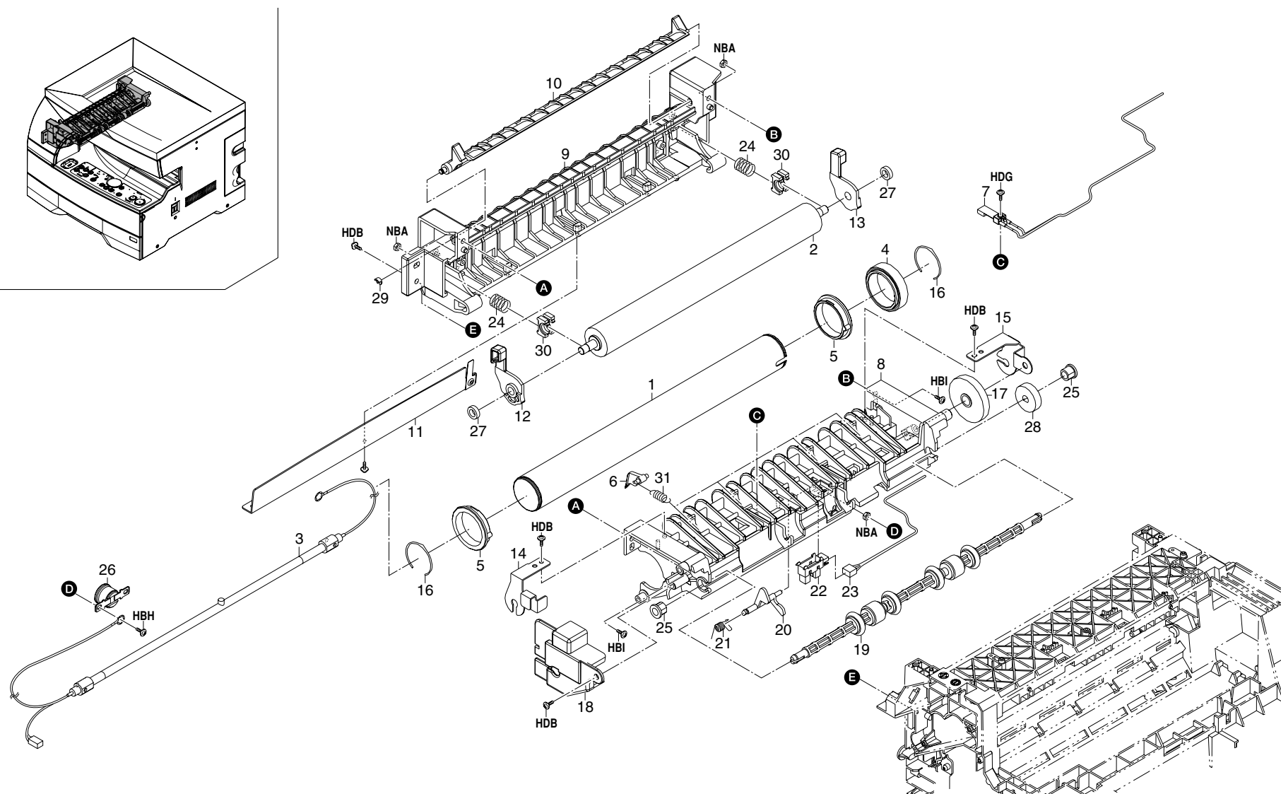
FIG. 12 FIXING SECTION
