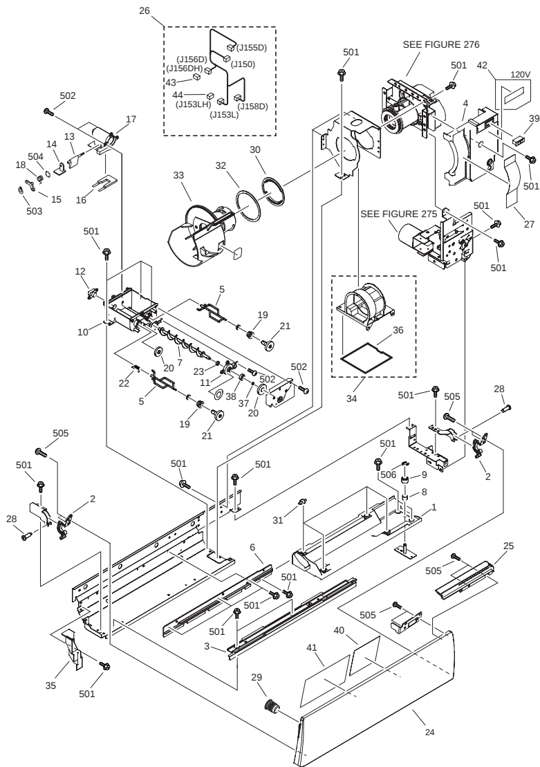
FIGURE 620 HOPPER ASSEMBLY
