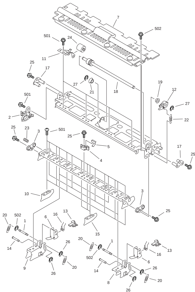
FIGURE 350 INTERNAL DELIVERY UPPER ASSEMBLY
