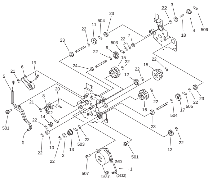
FIGURE 281 MAIN MOTOR DRIVE ASSEMBLY
