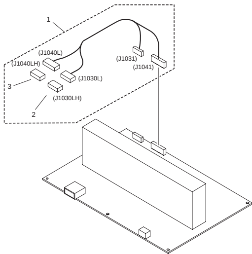
FIGURE 941 FIXING HEATER PS PCB ASSEMBLY
