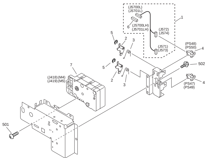
FIGURE 232 LIFTER DRIVE ASSEMBLY
