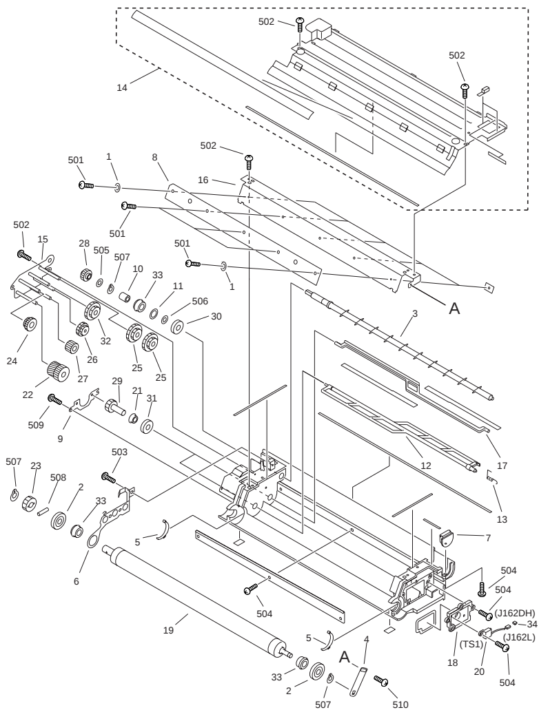
FIGURE 640 DEVELOPING ASSEMBLY
