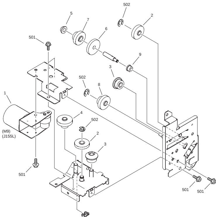
FIGURE 275 HOPPER DRIVE ASSEMBLY
