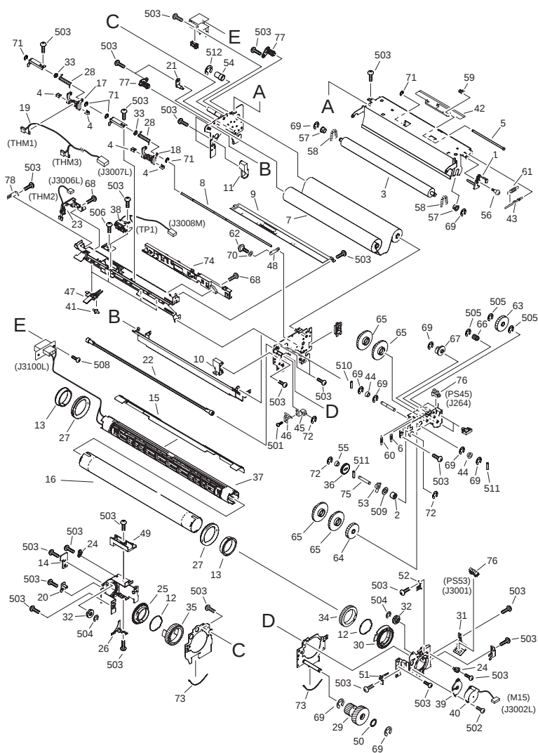
FIGURE 810 FIXING ASSEMBLY
