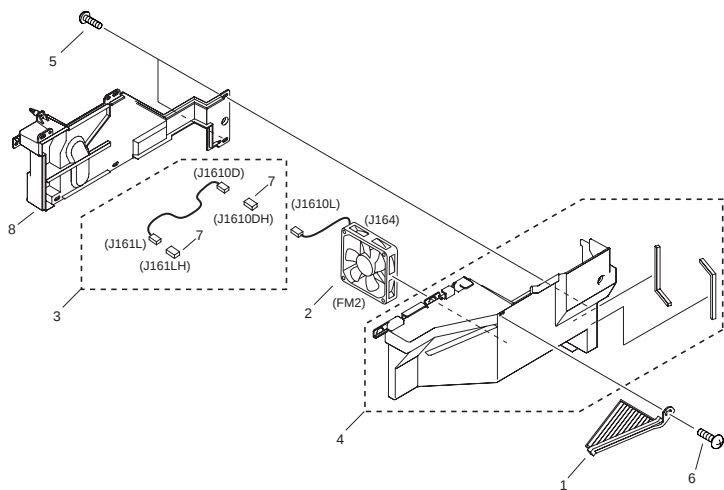
FIGURE 191 PRIMARY FAN DUCT ASSEMBLY
