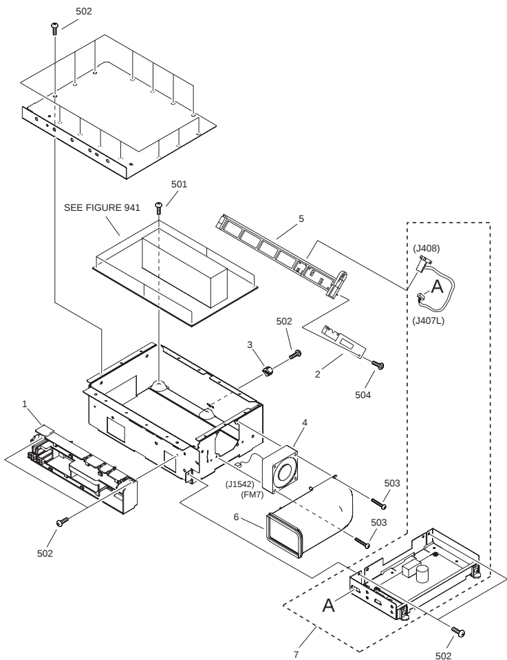
FIGURE 940 IH POWER/POTENTIAL SENSOR PCB ASSEMBLY
