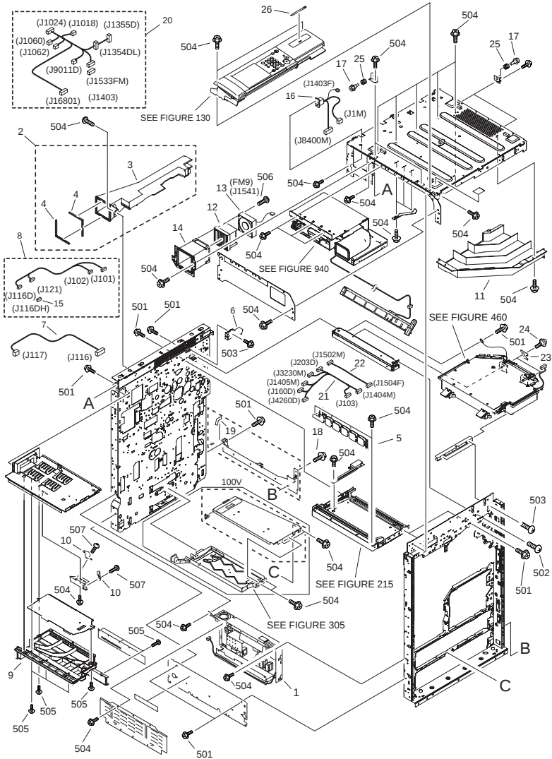
FIGURE 103 INTERNAL COMPONENTS 2
