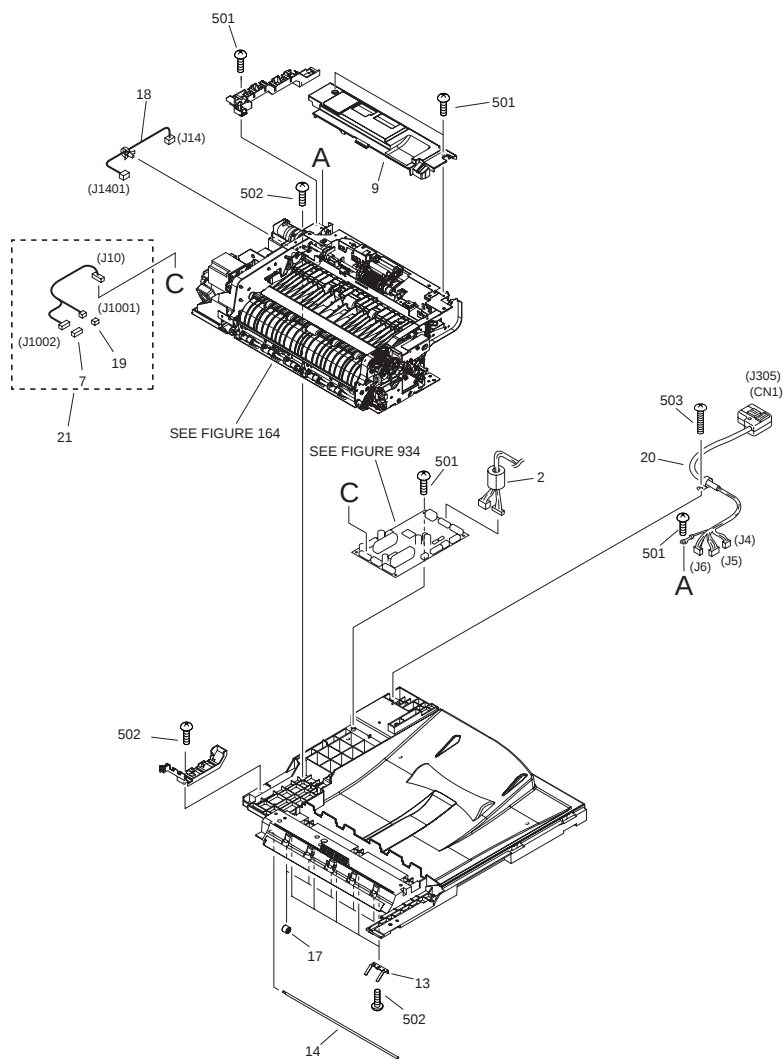
FIGURE 161 ADF ASSEMBLY
