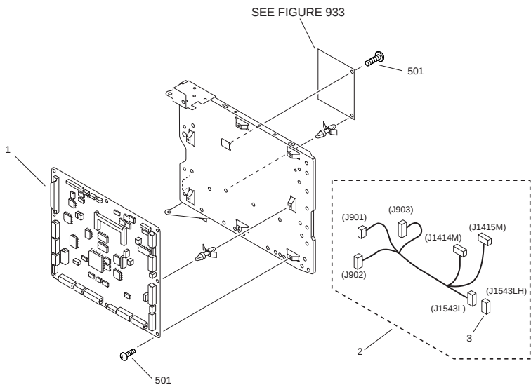
FIGURE 930 DC CONTROLLER PCB ASSEMBLY
