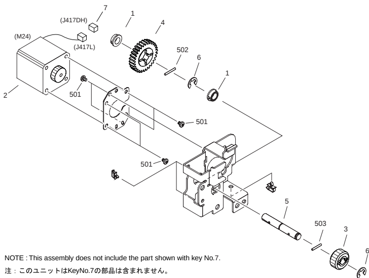
FIGURE 263 LEFT PICK-UP DRIVE ASSEMBLY
