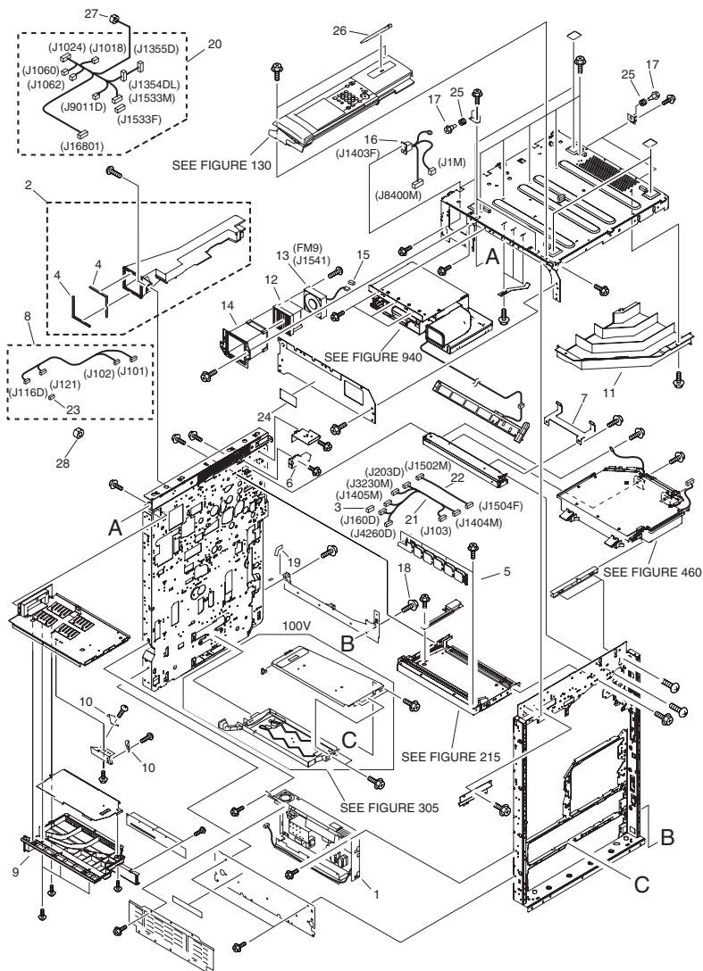
FIGURE 103 INTERNAL COMPONENTS 2
