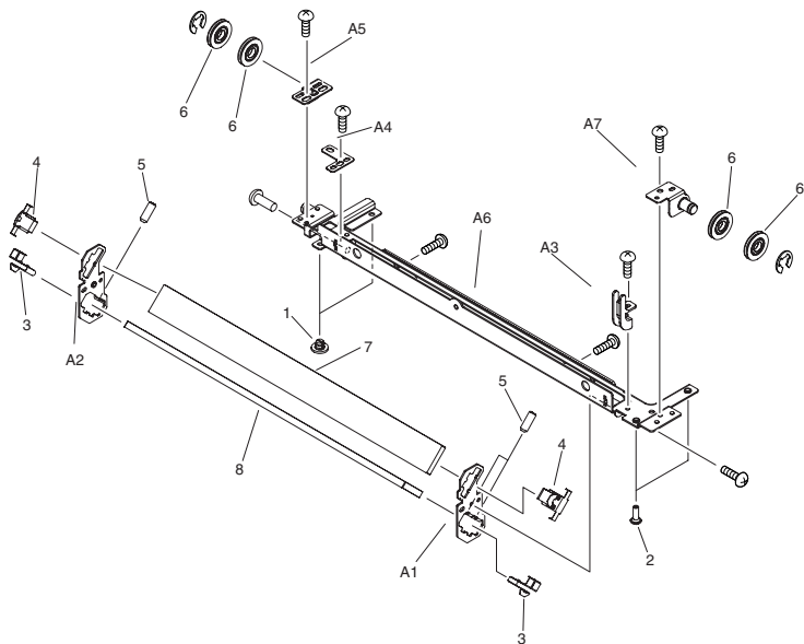
FIGURE 430 MIRROR ASSEMBLY 2
