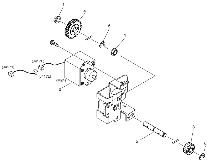
FIGURE 263 LEFT PICK-UP DRIVE ASSEMBLY
