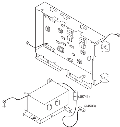
FIGURE 980 H.V. TRANSFORMER PCB ASSEMBLY(iR5055/5065)
