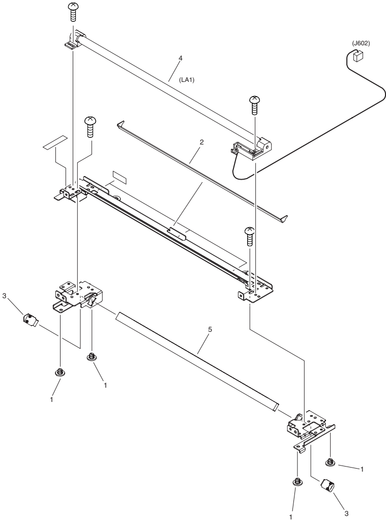
FIGURE 420 MIRROR ASSEMBLY 1
