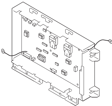
FIGURE 981 DC H.V. TRANSFORMER PCB ASSEMBLY(iR5075)
