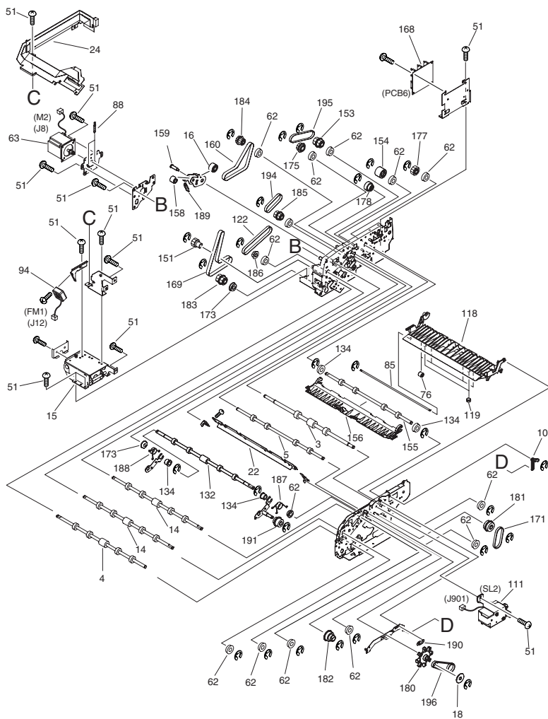
FIGURE A40 ADF PAPER FEEDER ASSEMBLY
