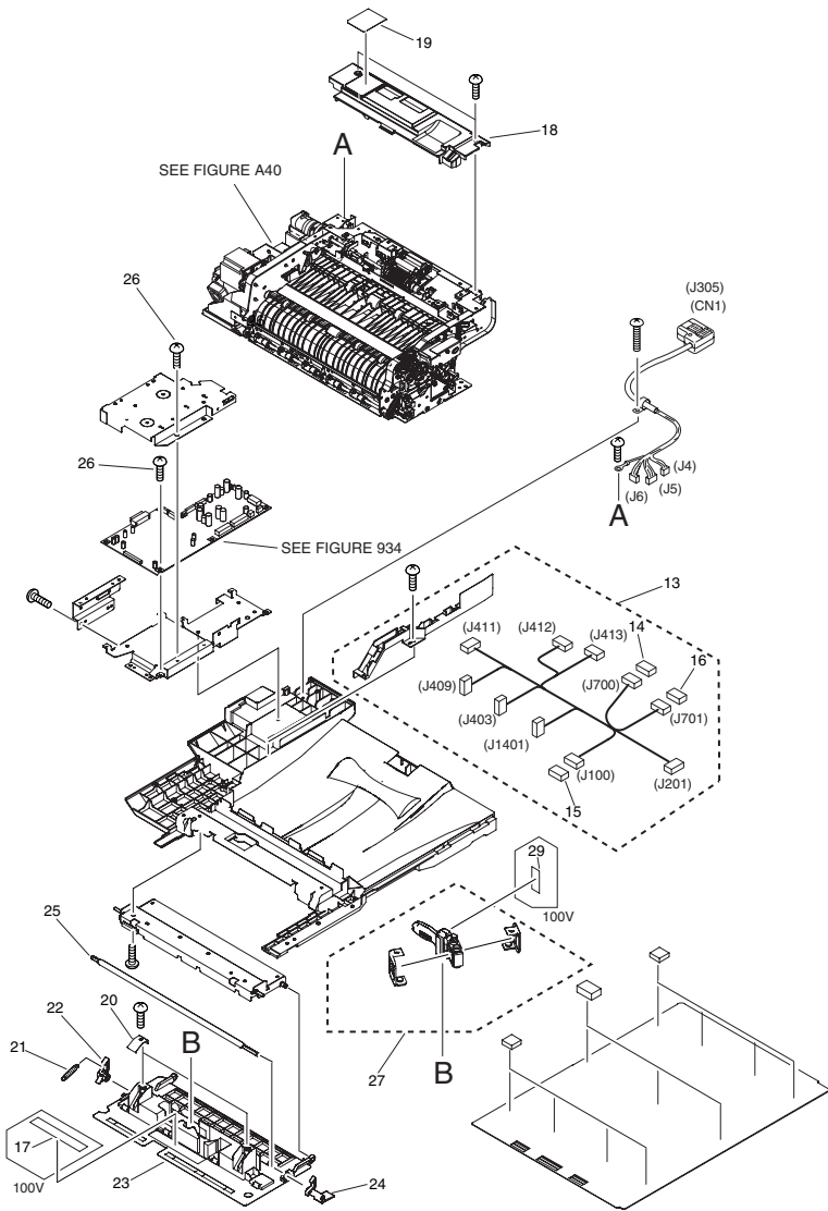
FIGURE A10 ADF ASSEMBLY
