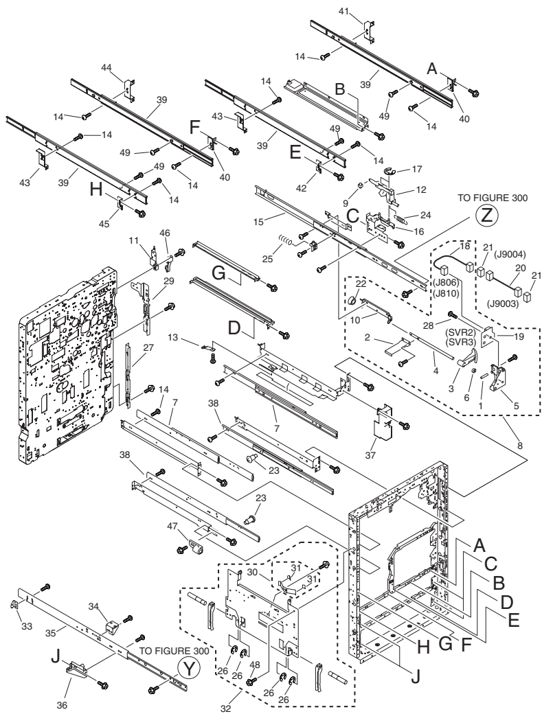
FIGURE 104 INTERNAL COMPONENTS 3
