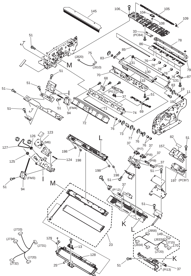
FIGURE A40 ADF PAPER FEEDER ASSEMBLY
