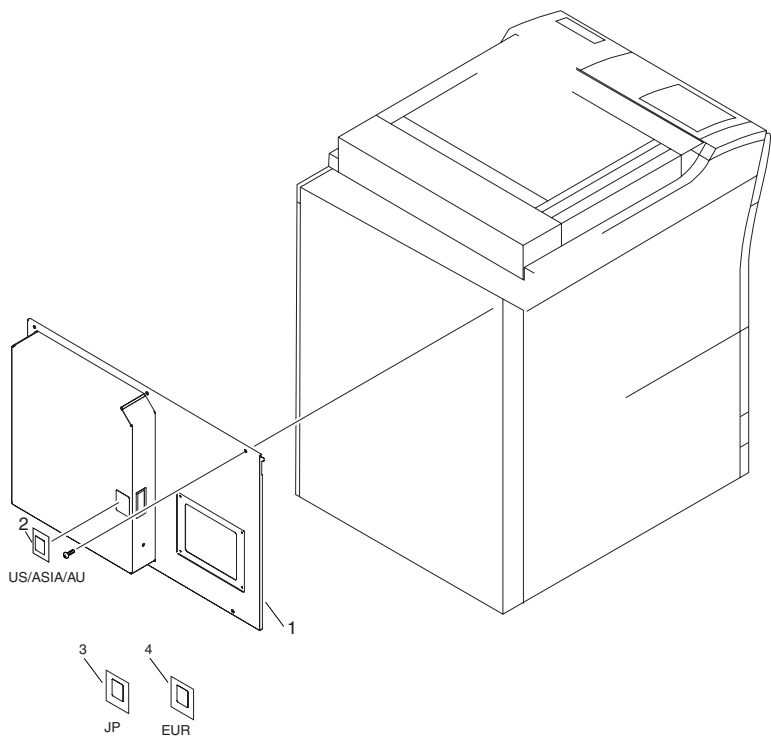
FIGURE T10 EXTERNAL COVERS, PANELS, ETC
