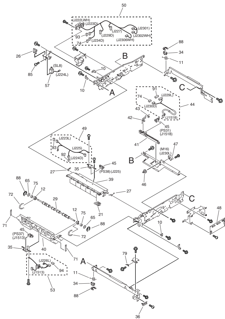
FIGURE 360 DUPLEXING FEEDER ASSEMBLY
