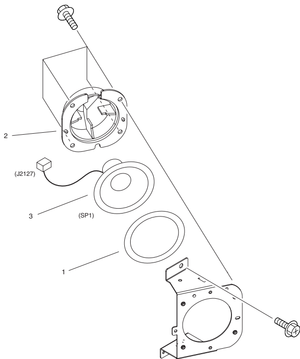
FIGURE T22 SPEAKER ASSEMBLY
