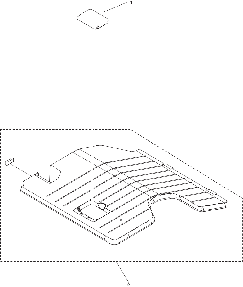
FIGURE Q22 2ND DELIVERY TRAY ASSEMBLY
