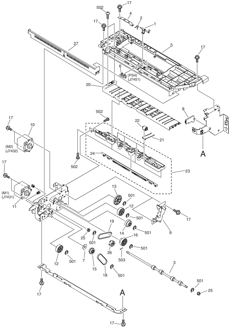
FIGURE Q37 2ND UPPER DELIVERY ASSEMBLY
