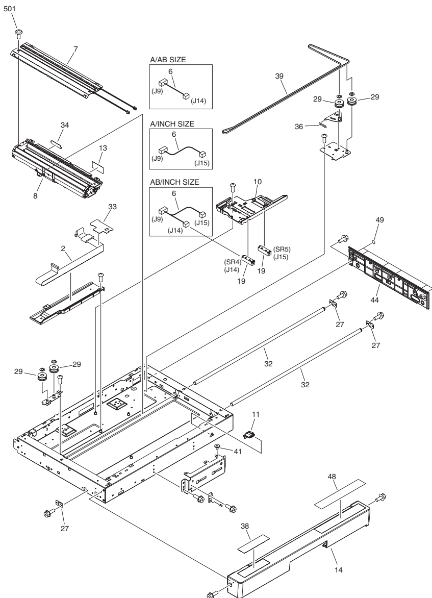
FIGURE 400 READER ASSEMBLY
