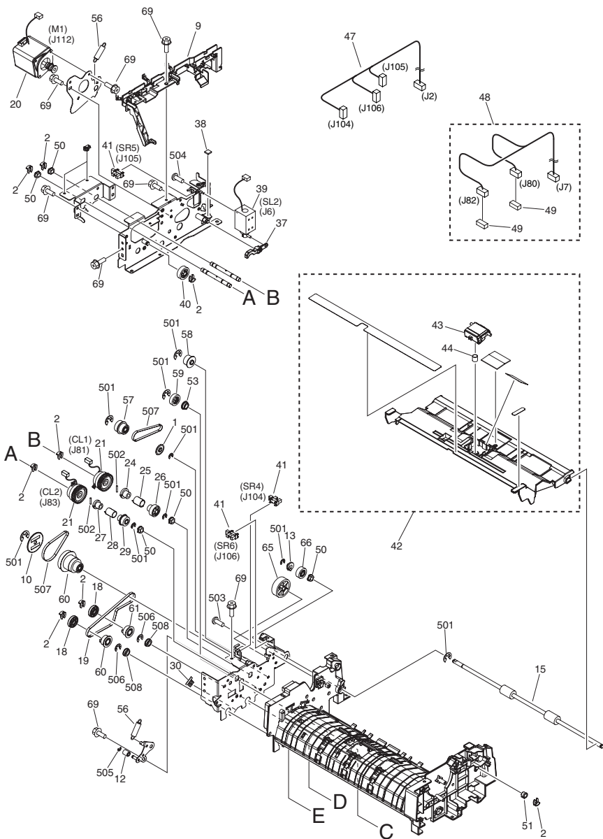
FIGURE A41 FEEDER ASSEMBLY
