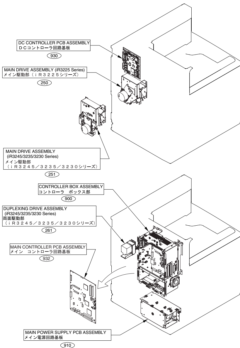
FIGURE A1 ASSEMBLY LOCATION DIAGRAM
