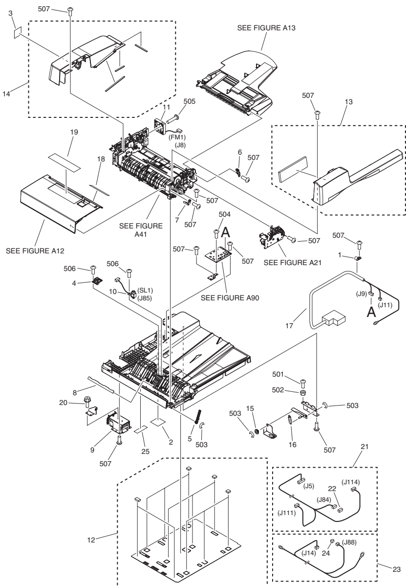
FIGURE A10 INTERNAL COMPONENTS
