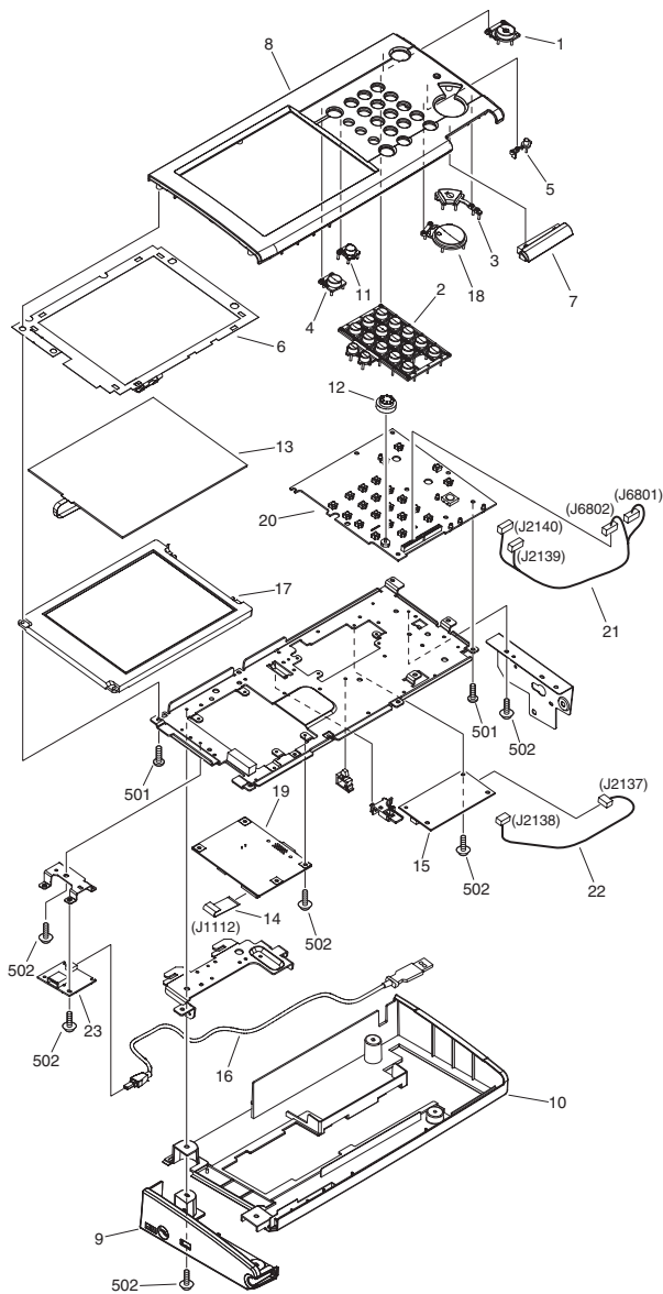
FIGURE 130 CONTROL PANEL ASSEMBLY
