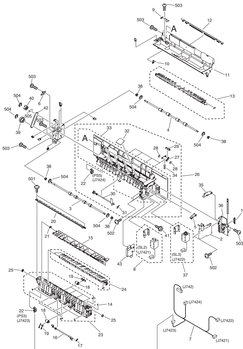
FIGURE Q39 3RD DELIVERY FRAME ASSEMBLY
