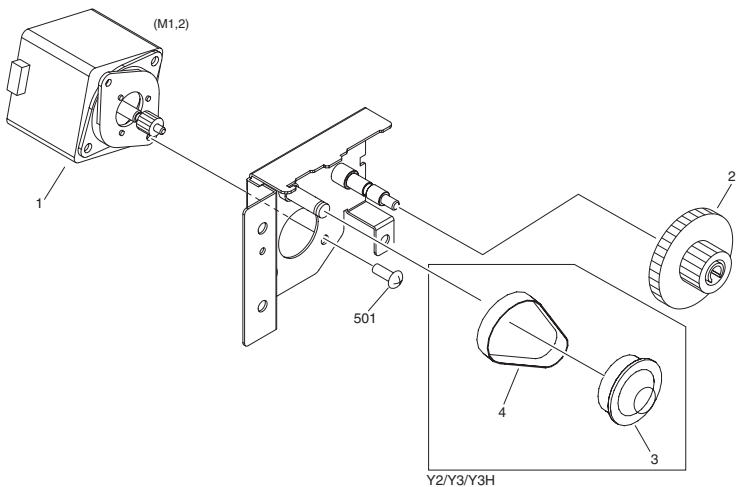
FIGURE Z20 DRIVE ASSEMBLY
