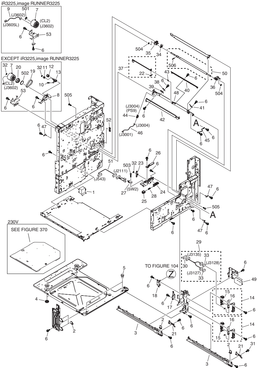
FIGURE 102 INTERNAL COMPONENTS 1
