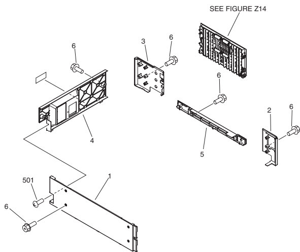
FIGURE Z10 EXTERNAL COVERS, PANELS, ETC.
