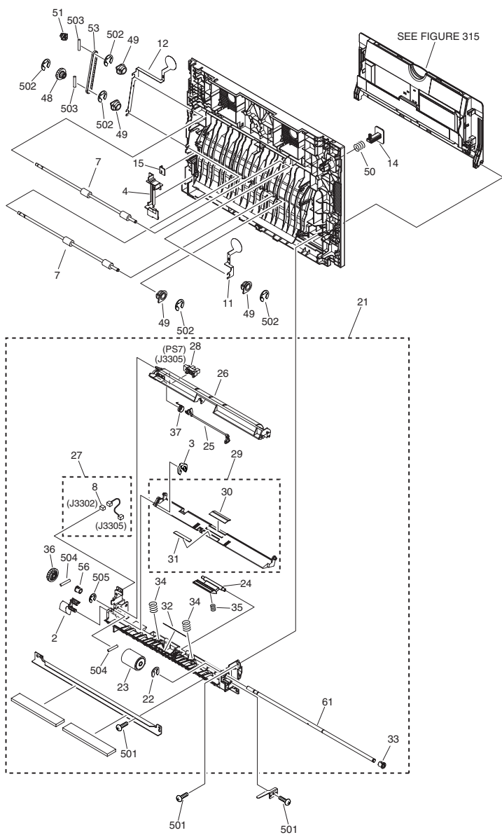
FIGURE 115 RIGHT DOOR ASSEMBLY
